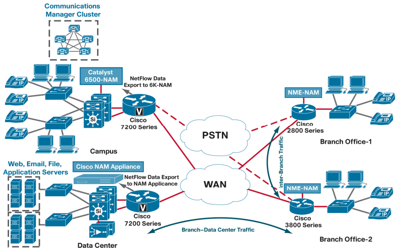
Figure 2. Deploying Cisco Branch Routers Series NAM to Build Intelligence into the Empowered Branch
