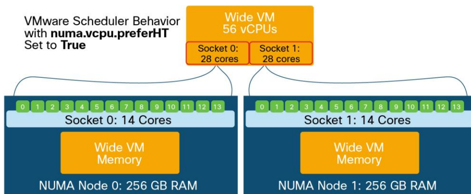
Figure 5. Wide Virtual Machine CPU Scheduling
