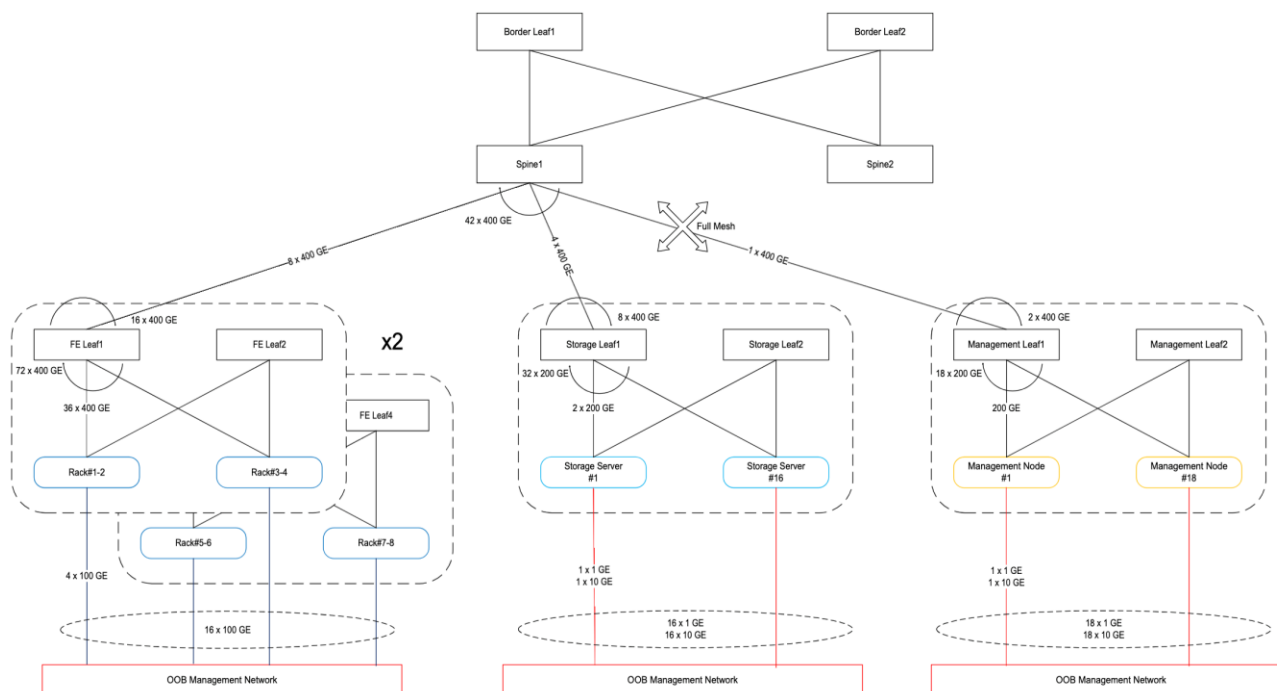
Figure 17. Converged North-South Storage and Management Network for 8 GB300 racks (576 GPUs)
