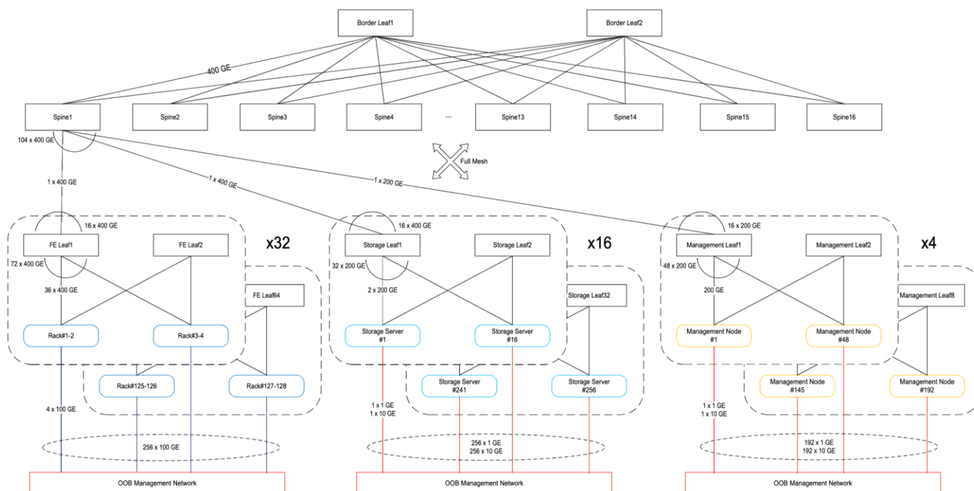
Figure 20. Converged North-South Storage and Management Network for 128 GB300 racks (9216 GPUs)
