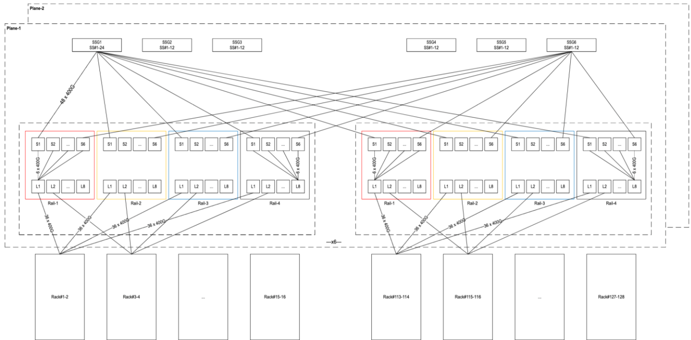
Figure 13. East-West three-tier Compute Network for 128 GB300 racks (9216 GPUs)
