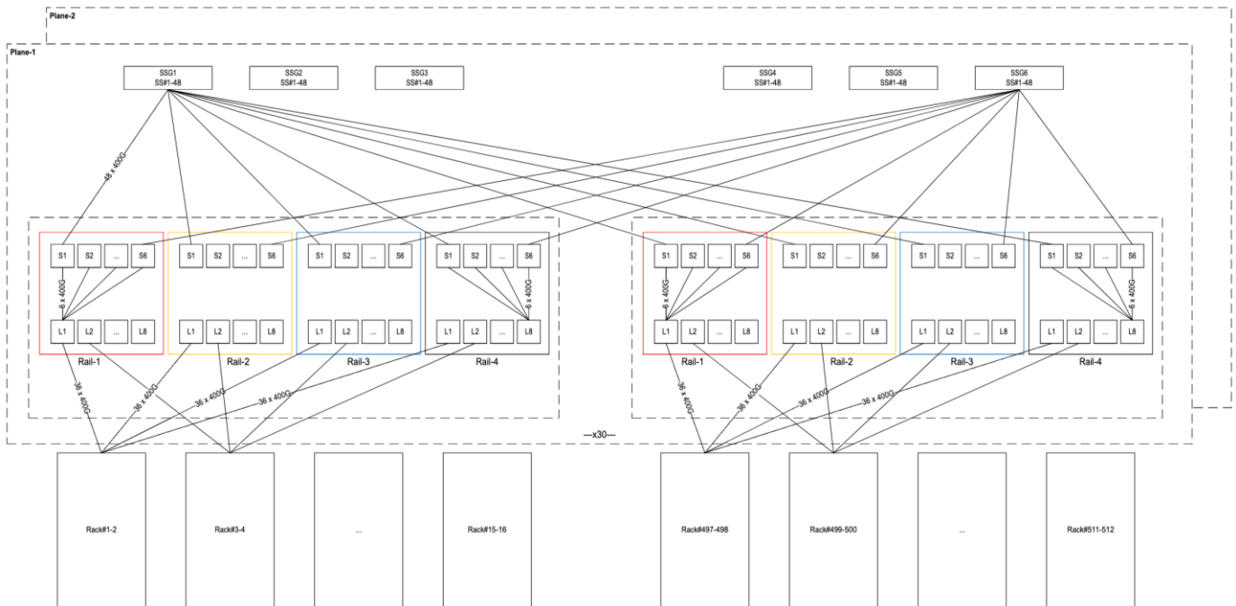
Figure 14. East-West three-tier Compute Network for 512 GB300 racks (36864 GPUs)
