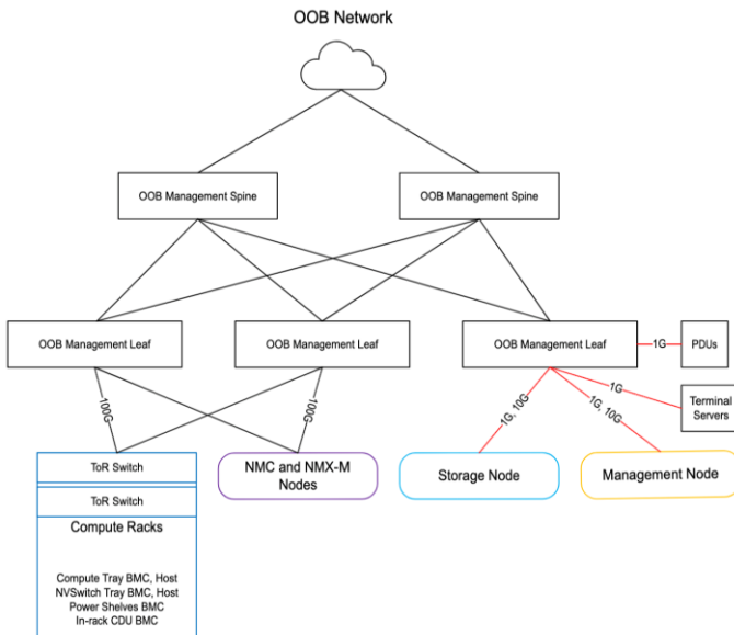
Figure 23. OOB Management Network
