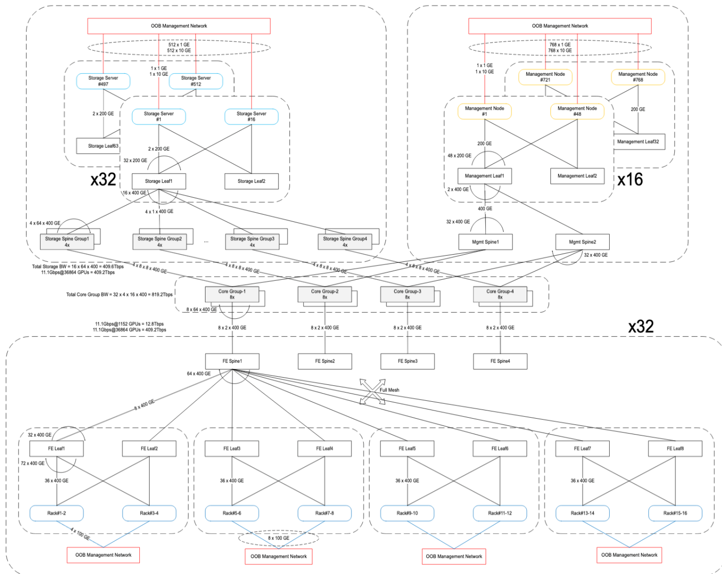
Figure 22. Converged North-South Storage and Management Network for 512 GB300 nodes (36864 GPUs)
