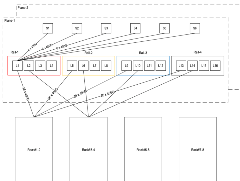
Figure 10. East-West two-tier Compute Network for 8 GB300 racks (576 GPUs)
