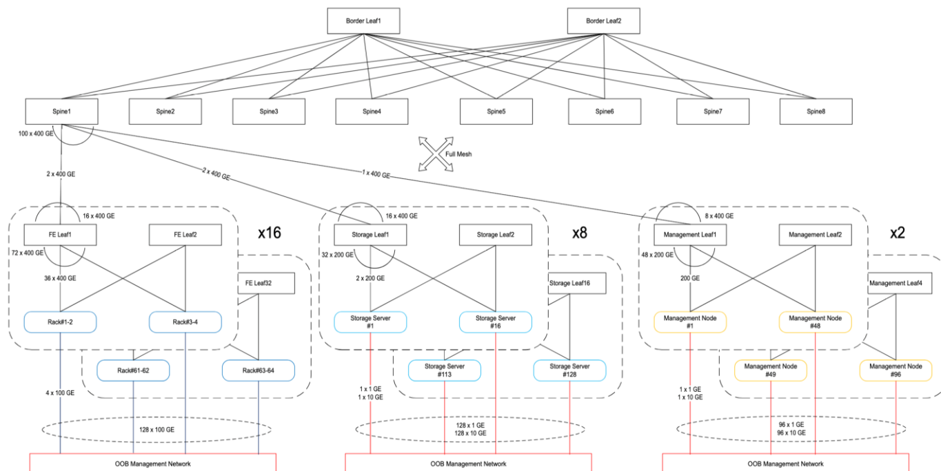
Figure 19. Converged North-South Storage and Management Network for 64 GB300 racks (4608 GPUs)
