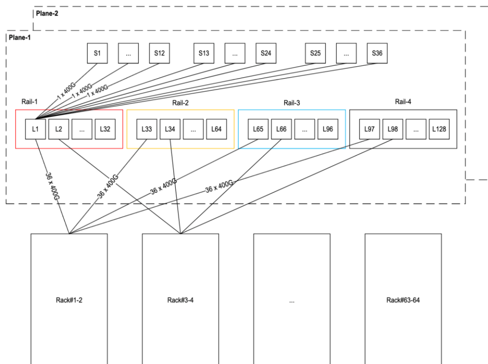
Figure 12. East-West two-tier Compute Network for 64 GB300 racks (4608 GPUs)
