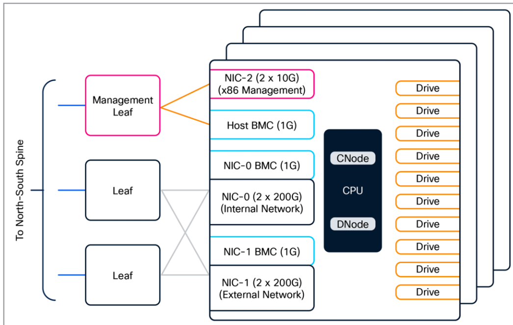
Figure 24. Cisco EBox Storage Logical Block Diagram
