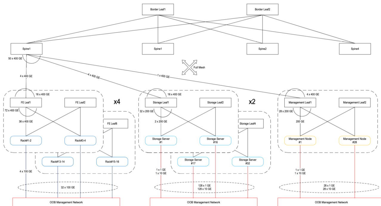
Figure 18. Converged North-South Storage and Management Network for 16 GB300 racks (1152 GPUs)
