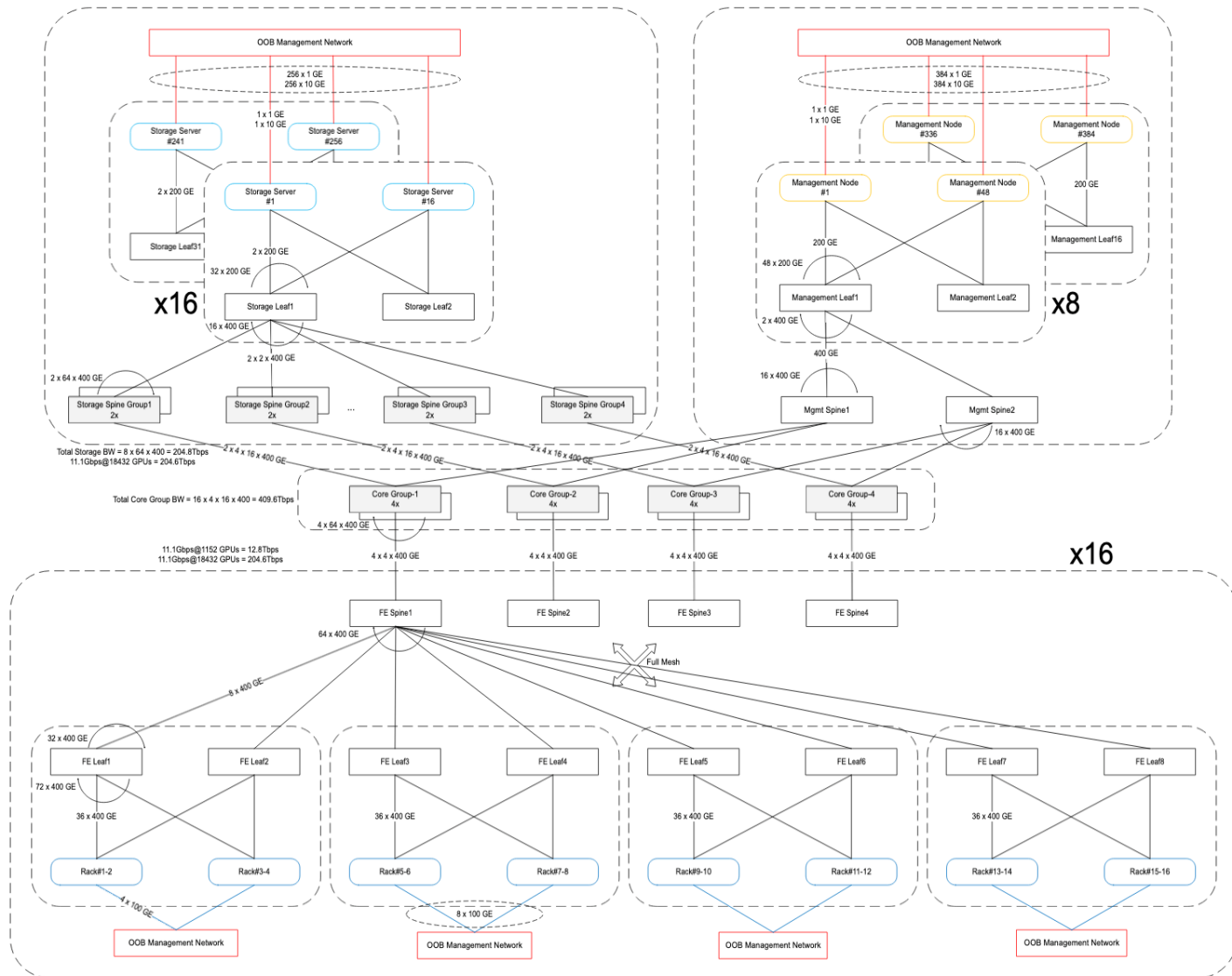
Figure 21. Converged North-South Storage and Management Network for 256 GB300 nodes (18432 GPUs)
