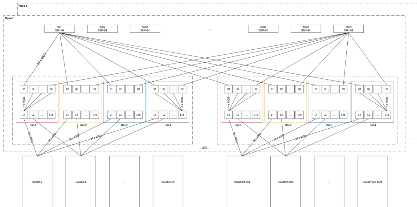
Figure 15. East-West three-tier Compute Network for 1024 GB300 racks (73728 GPUs)
