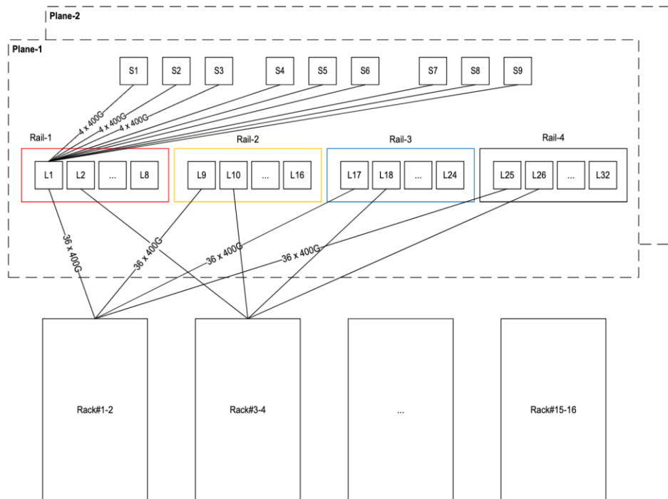
Figure 11. East-West two-tier Compute Network for 16 GB300 racks (1152 GPUs)
