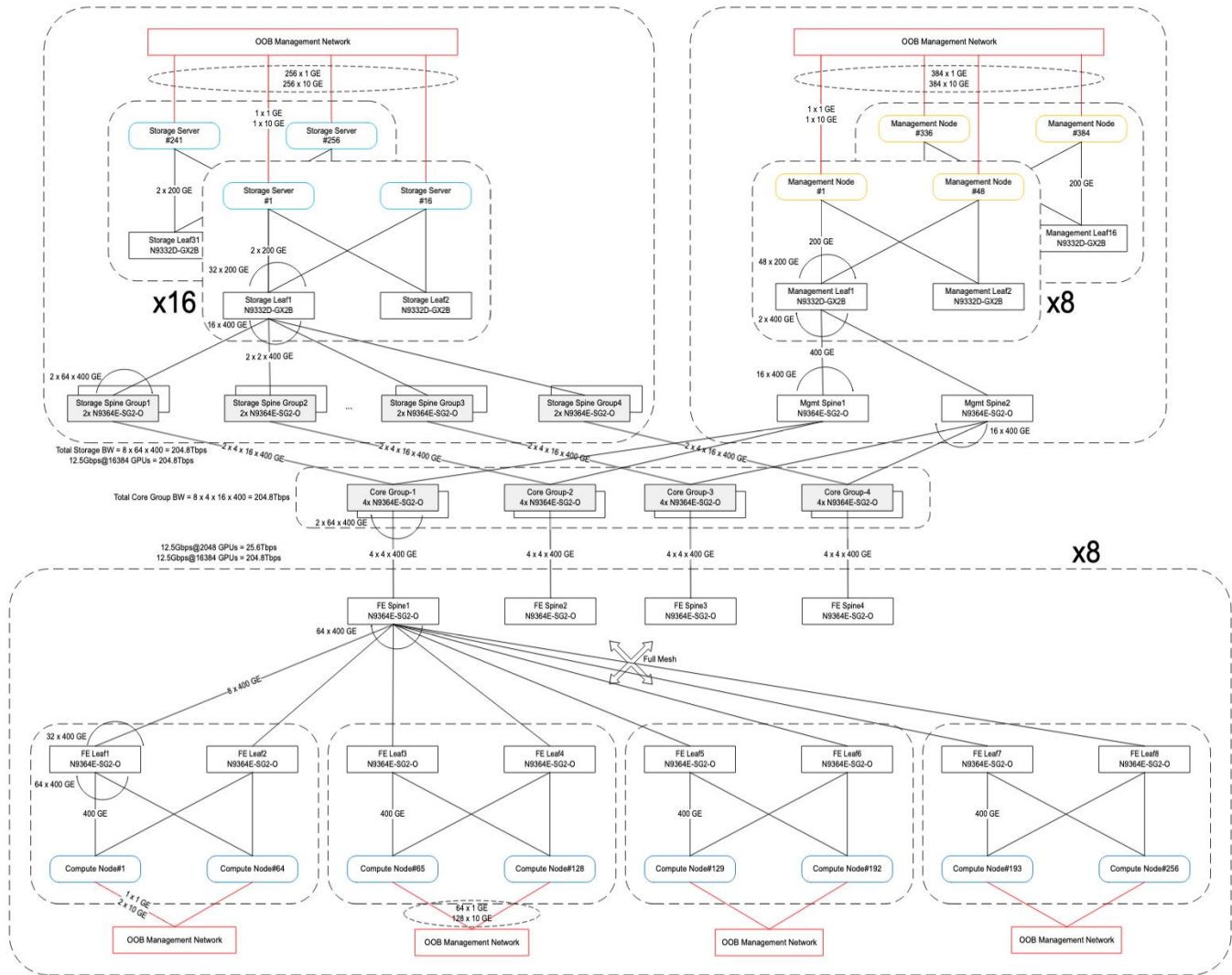
Figure 15. Converged North-South Storage and Management Network for 2048 HGX™ B300 nodes (16K GPUs)
