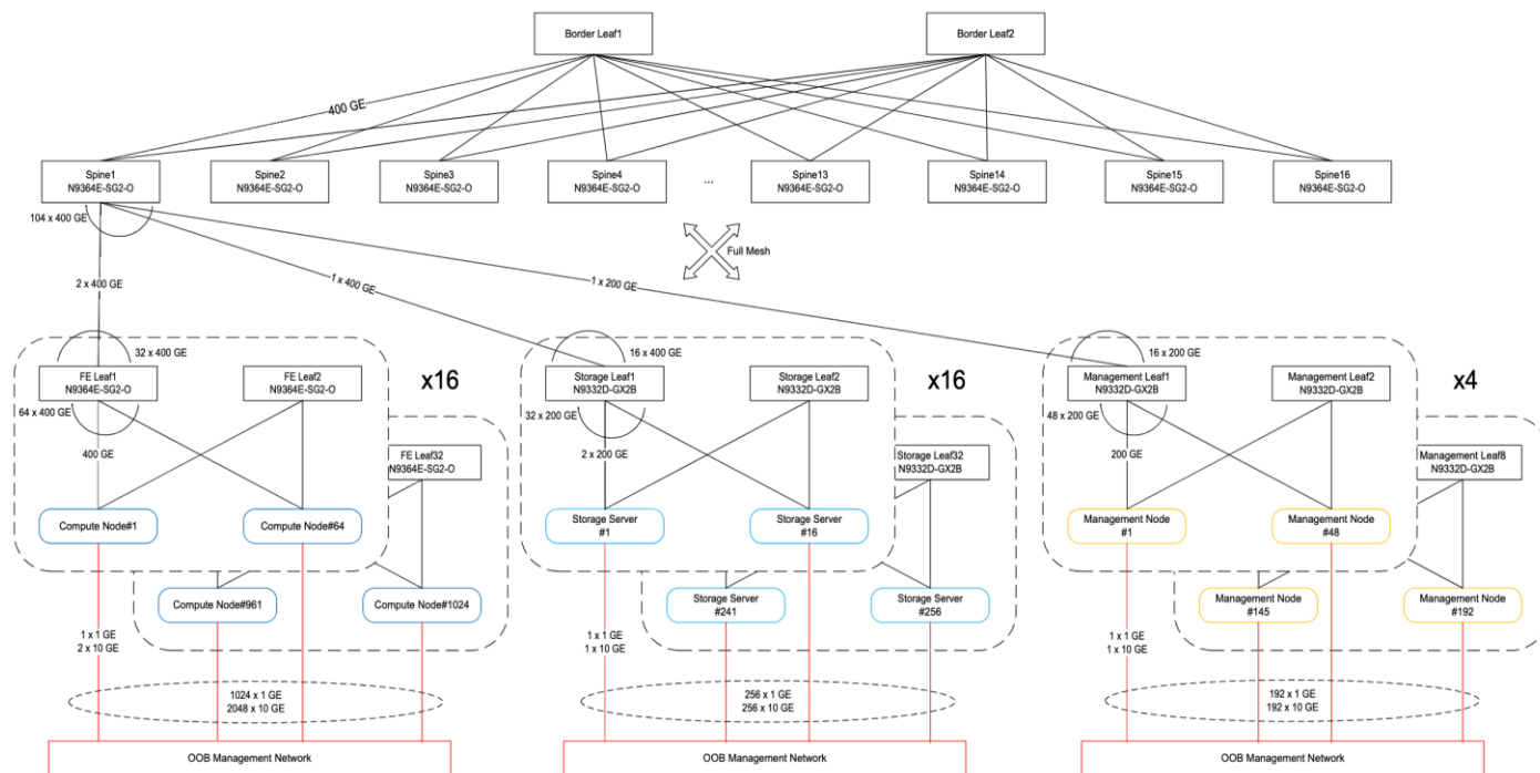
Figure 14. Converged North-South Storage and Management Network for 1024 HGX™ B300 nodes (8K GPUs)
