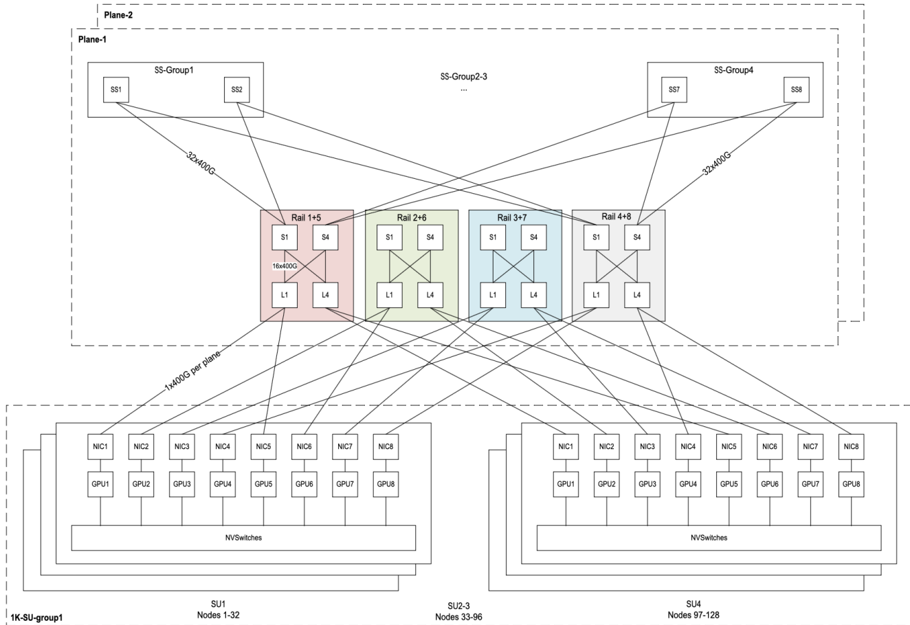
Figure 10. East-West three-tier Compute Network for 128 HGX™ B300 nodes (1K GPUs)
