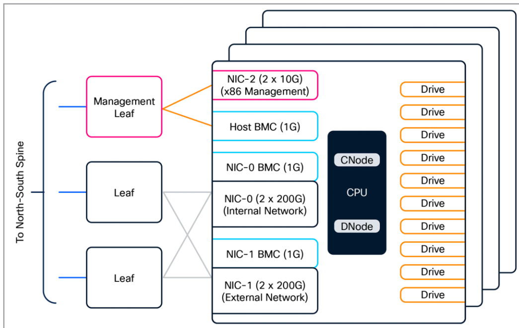
Figure 18. Cisco EBox Storage Logical Block Diagram
