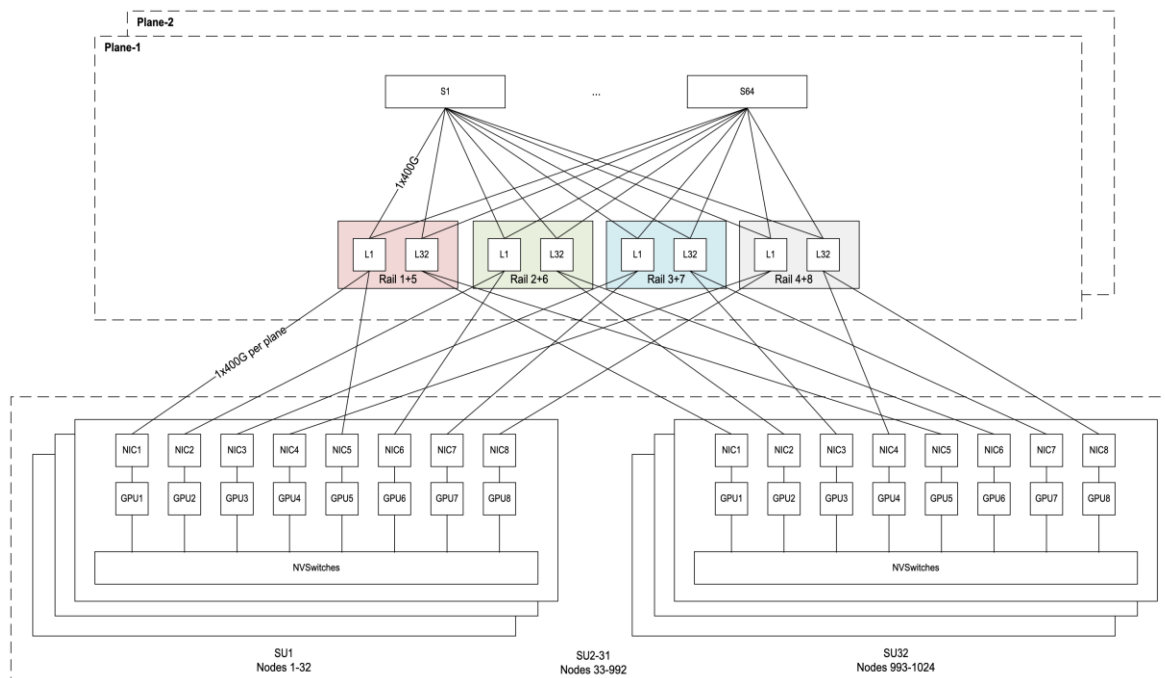
Figure 9. East-West two-tier Compute Network for 1024 HGX™ B300 nodes (8K GPUs)
