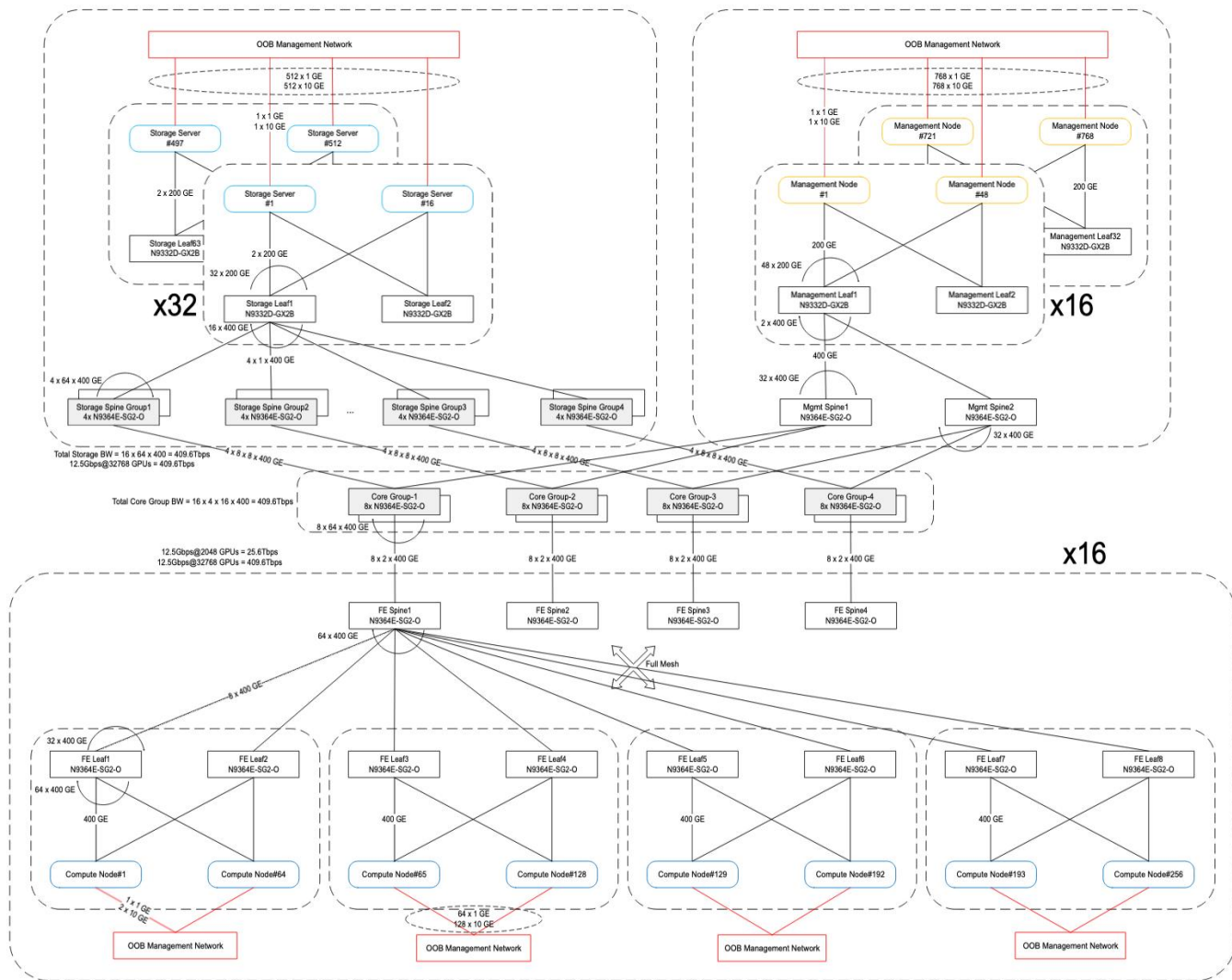
Figure 16. Converged North-South Storage and Management Network for 4096 HGX™ B300 nodes (32K GPUs)
