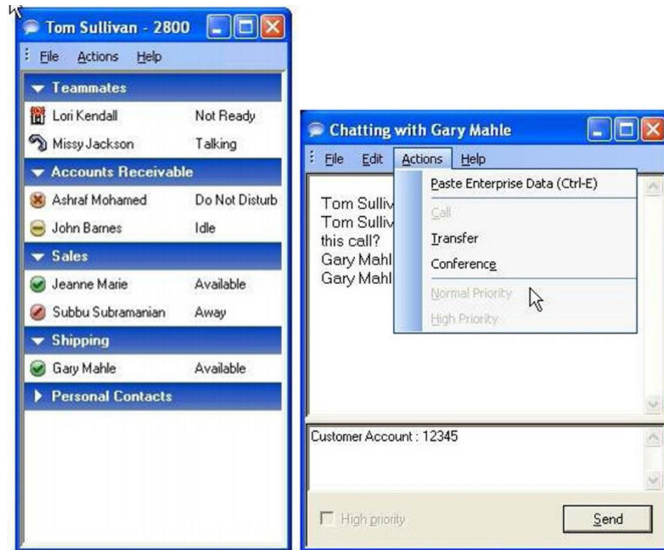
Figure 2. Desktop Contact Selection and Chat Windows
