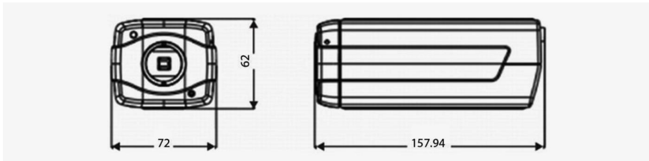
Figure 2. Cisco Video Surveillance 8000P IP Camera dimensions
