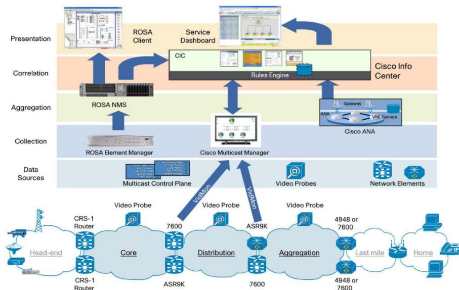
Figure 1. Cisco VAMS 3.1 Solution Architecture
