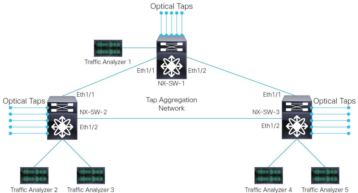
Figure 1. Monitoring Network Topology
