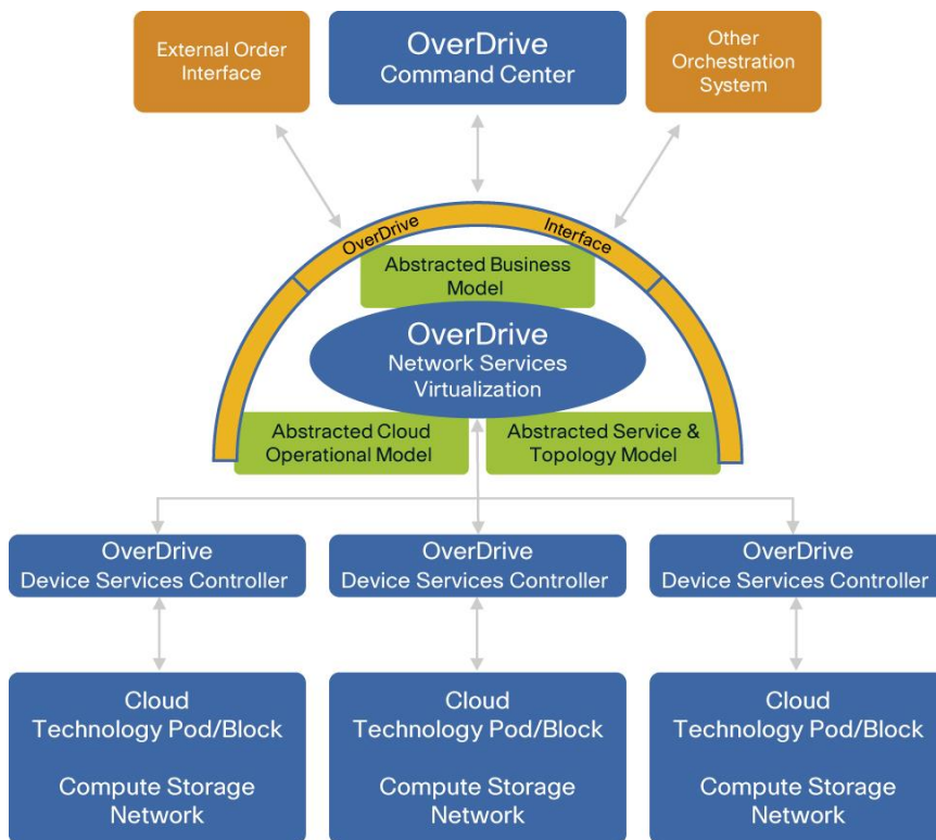
Figure 3. OverDrive Network Hypervisor Architecture
