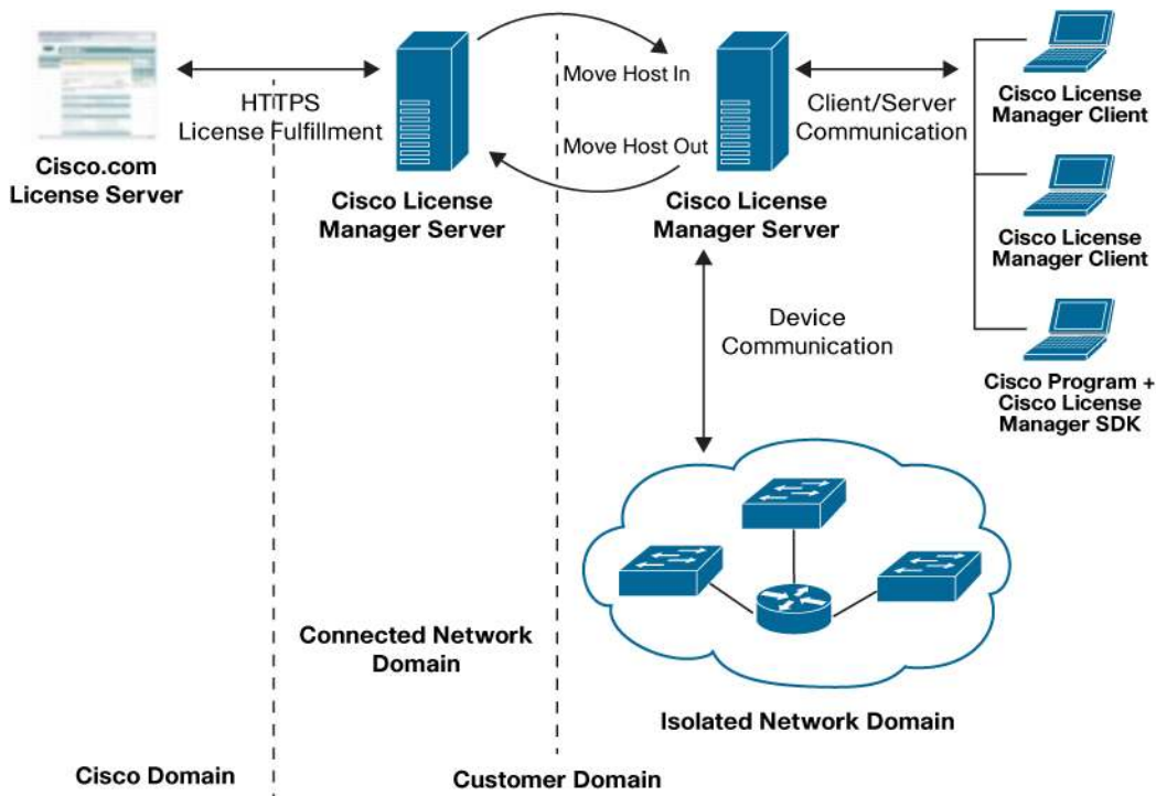
Figure 1. Two-Stage Deployment Diagram
