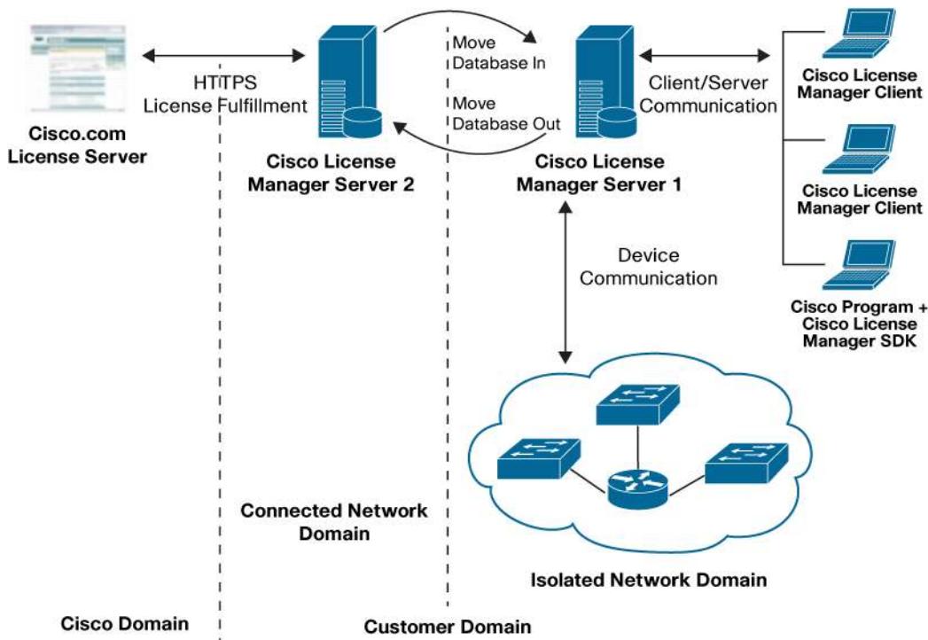
Figure 2. Two-Host Deployment Diagram
