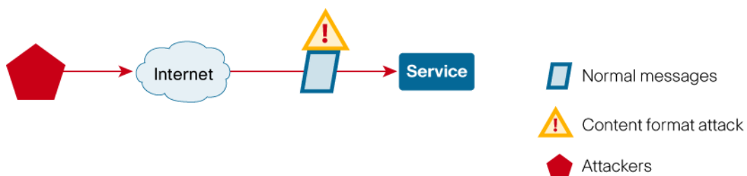
Figure 5. Content Format
