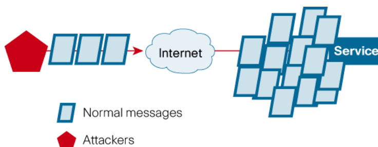
Figure 6. XDoS Attack
