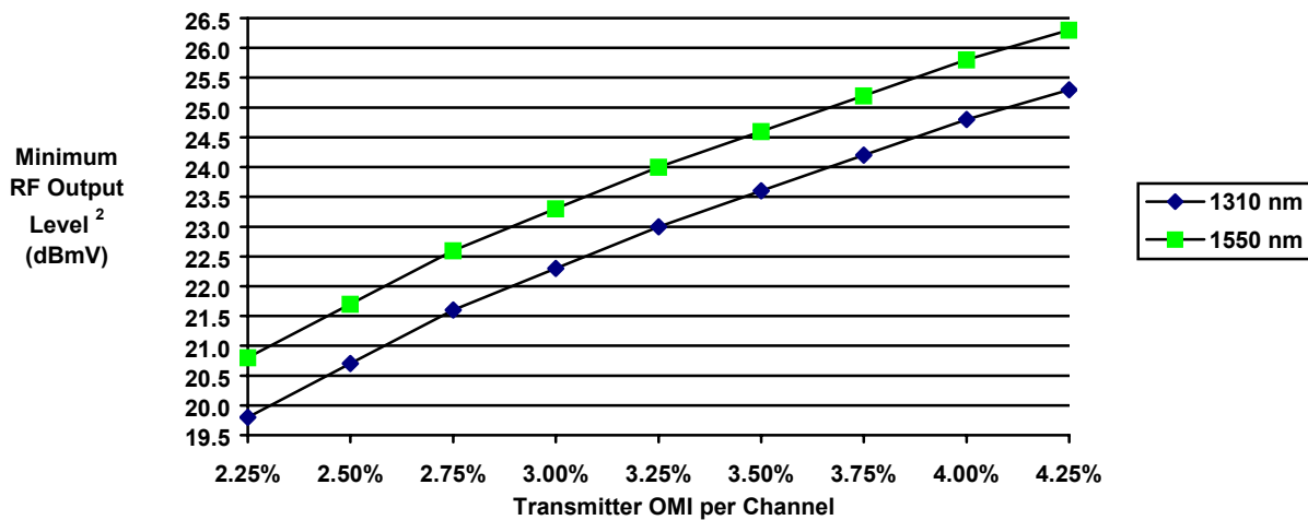
Receiver RF Output Level Vs Transmitter OMI (using Standard Receiver)
