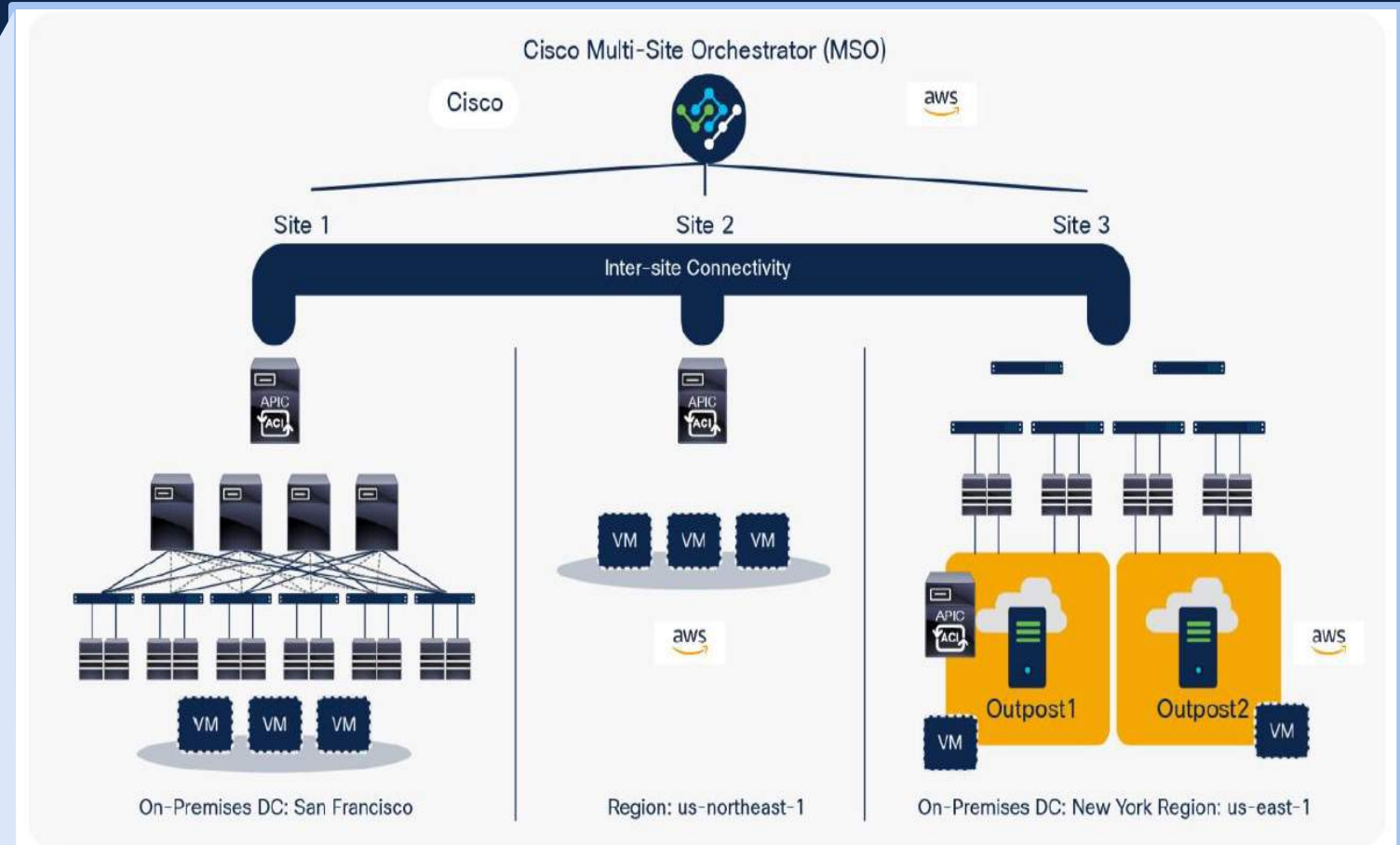
Figure 6. ACI extensions to hybrid cloud and AWS Outposts
