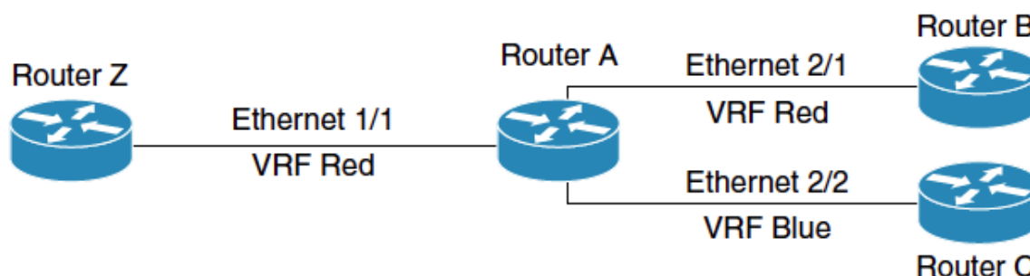
Figure 1 VRFs in a Network
