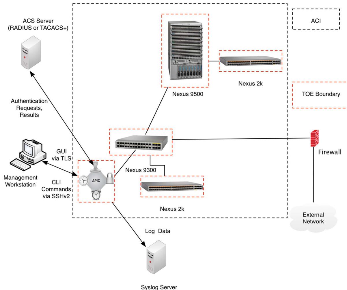
Figure 3 TOE and Environment Components
