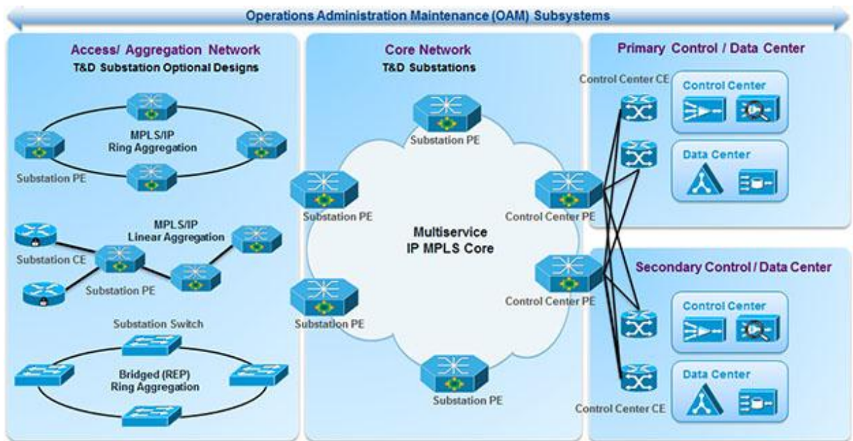
Figure 1. MPLS architectural configuration options
