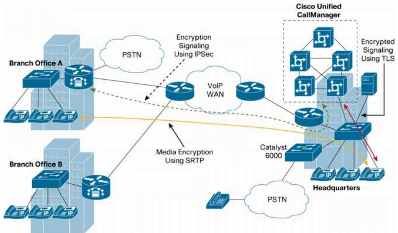
Figure 4: Media Authentication and Encryption in Cisco ISR Routers
