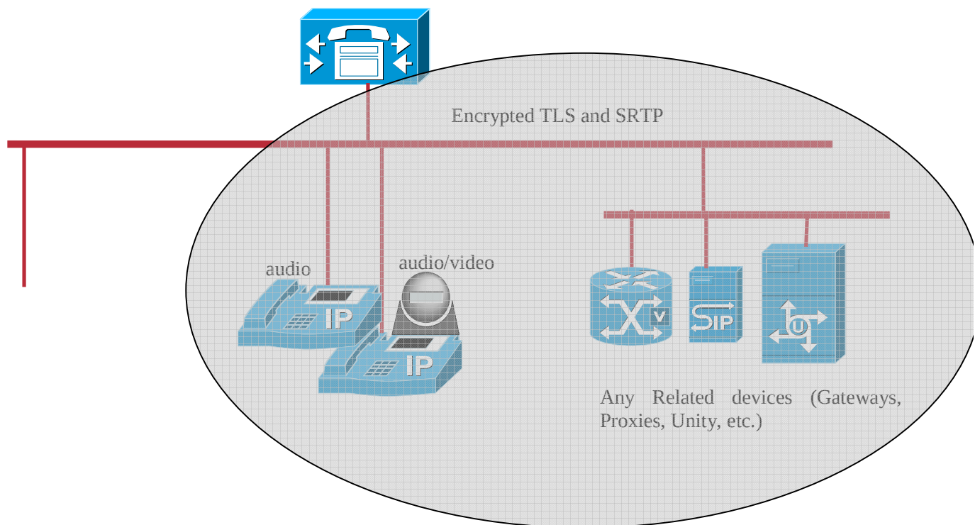
Figure 3: Example of encryptions in Cisco Call Manager
