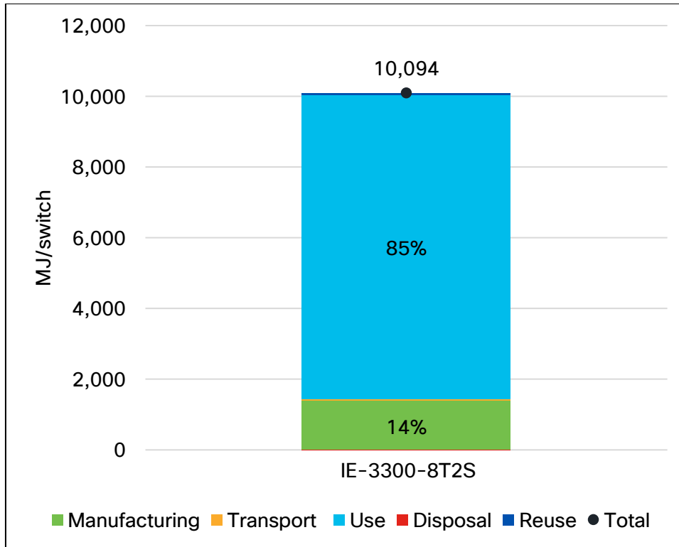
Figure 5: Primary Energy Demand per IE-3300-8T2S by Life Cycle Stage
