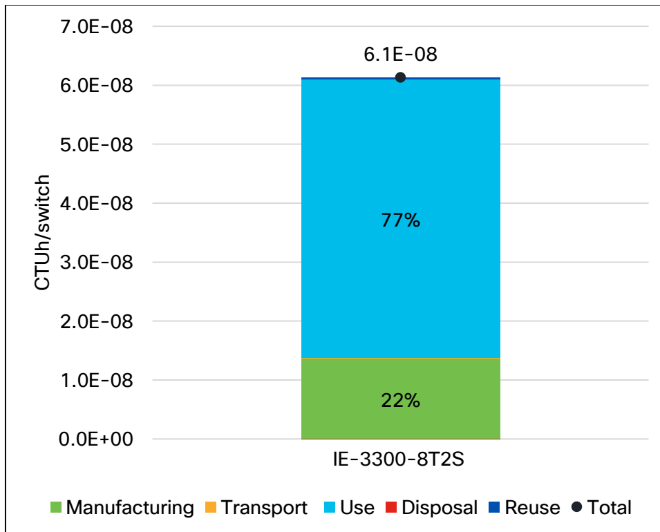
Figure 9: Human Toxicity (Cancer) per IE-3300-8T2S by Life Cycle Stage
