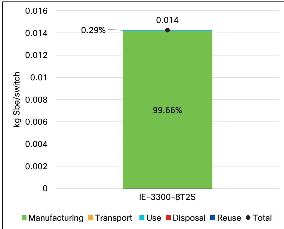
Figure 7: Abiotic Depletion Potential per IE-3300-8T2S by Life Cycle Stage
