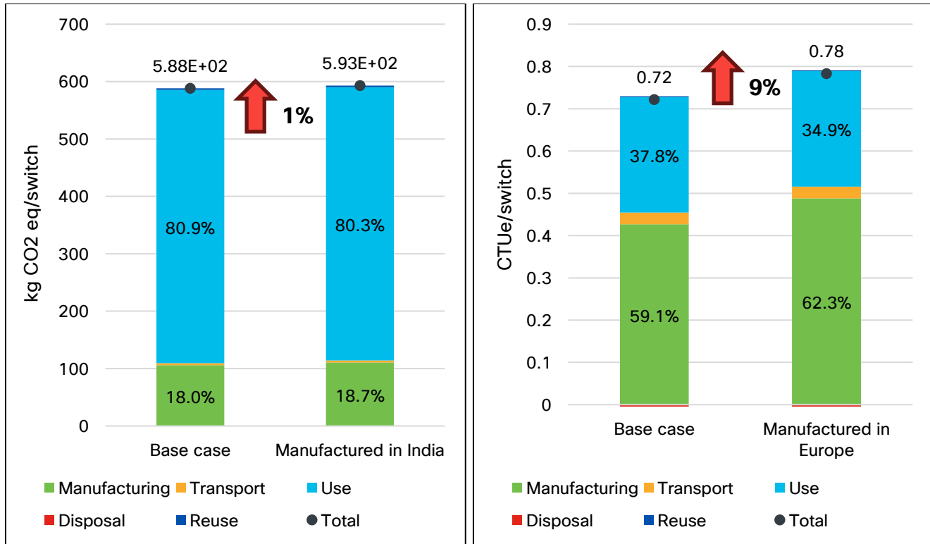
Figure 11: Sensitivity Analysis Results for GWP and Ecotoxicity with IE-3300-8T2S manufactured in India
