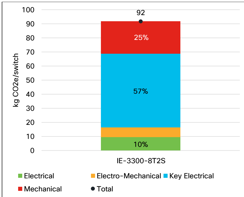
Figure 4: Global Warming Potential per IE-3300-8T2S from Manufacturing Components Across the Upstream Supply Chain
