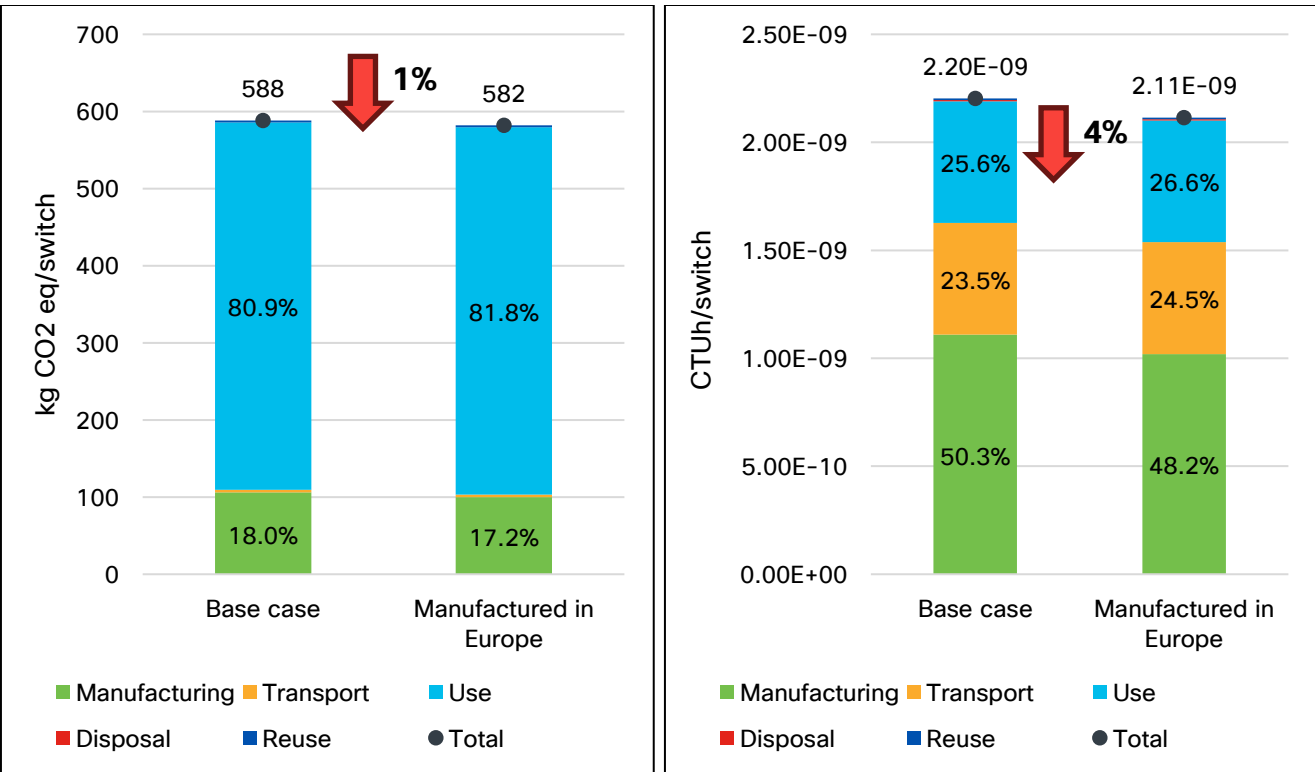
Figure 12: Sensitivity Analysis Results for GWP and Human Toxicity (non-cancer) with IE-3300-8T2S manufactured in Europe
