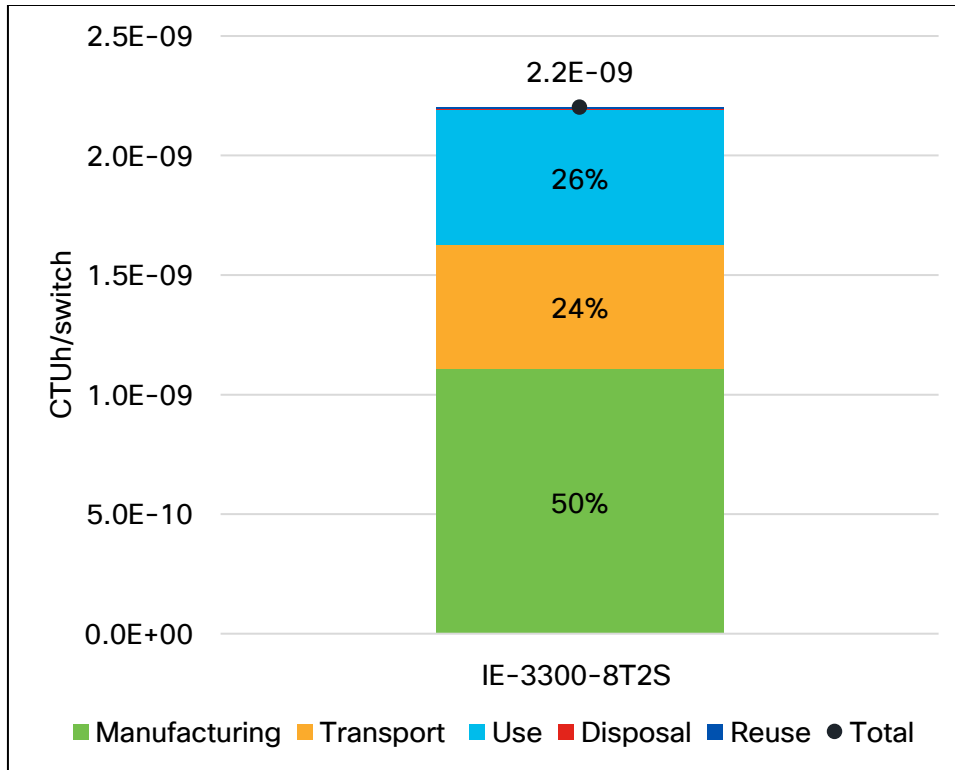
Figure 10: Human Toxicity (Non-Cancer) per IE-3300-8T2S by Life Cycle Stage
