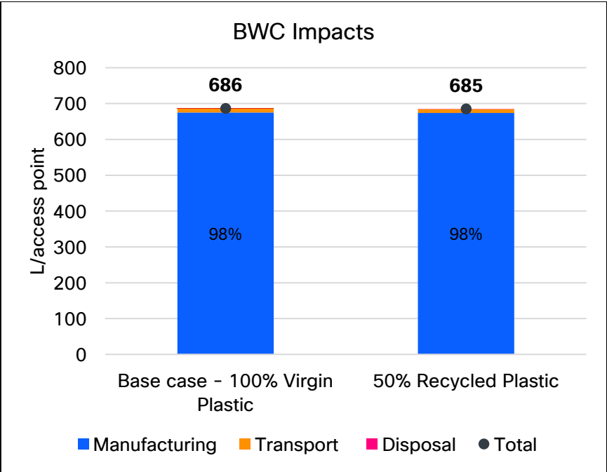
Figure 9: BWC Sensitivity Analysis Results for CW9171I access point excluding Use Phase
