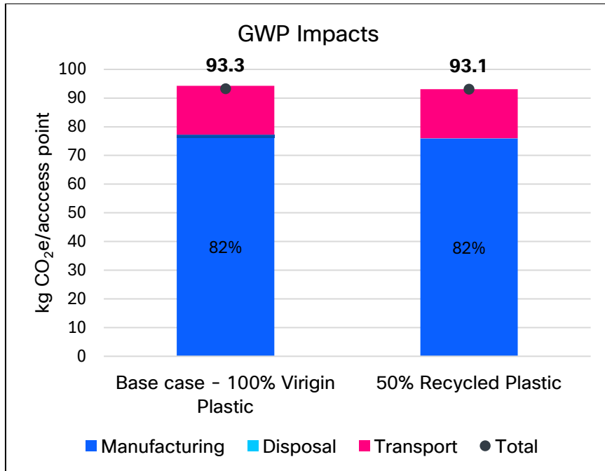
Figure 8: GWP Sensitivity Analysis Results for CW9171I access point excluding Use Phase
