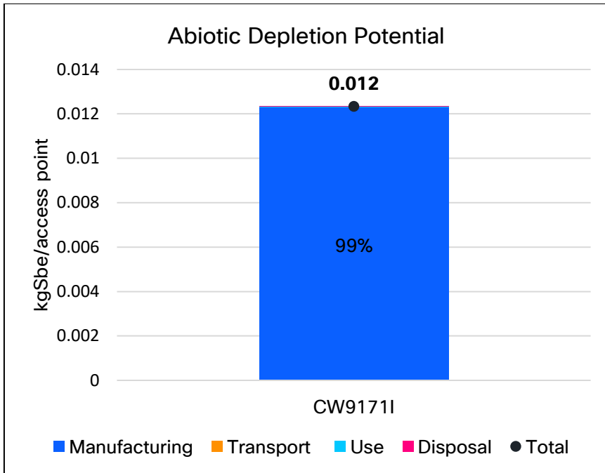
Figure 7: Abiotic Depletion Potential per CW9171I access point by Life Cycle Stage
