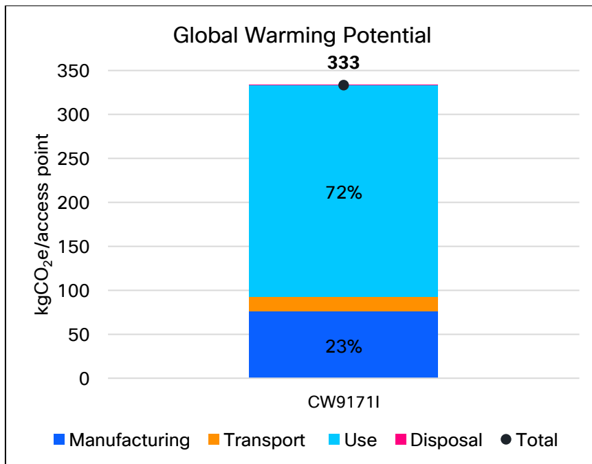
Figure 3: Global Warming Potential per CW9171I Access Point by Life Cycle Stage
