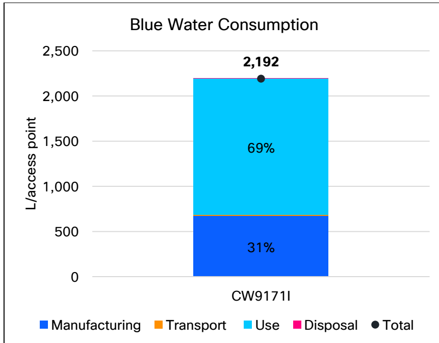
Figure 6: Blue Water Consumption per CW9171I access point by Life Cycle Stage
