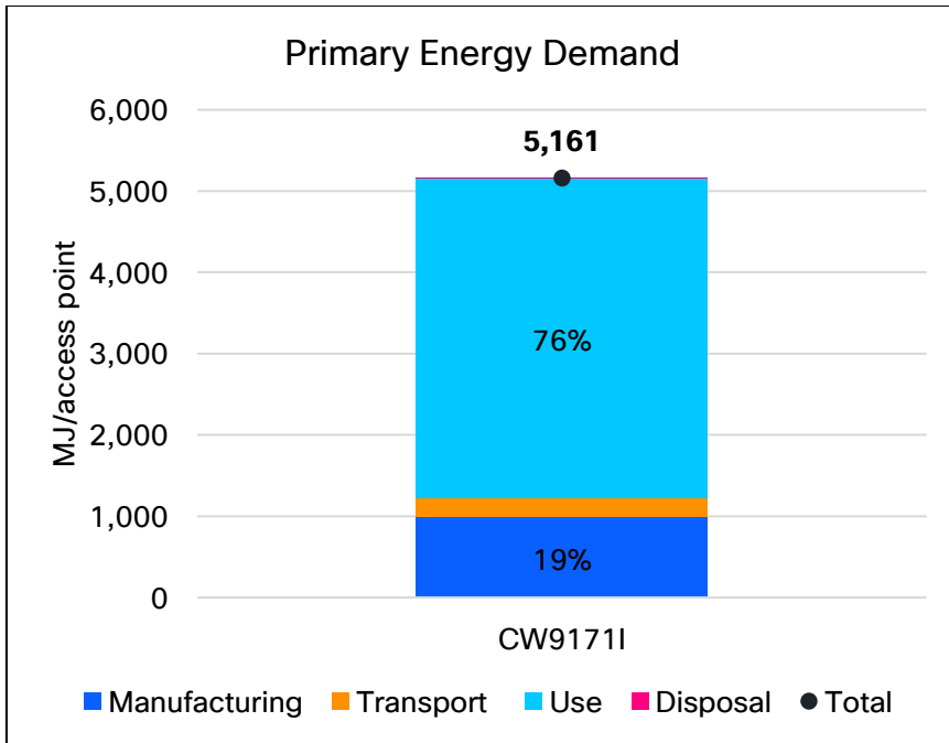
Figure 5: Primary Energy Demand per CW9171I access point by Life Cycle Stage
