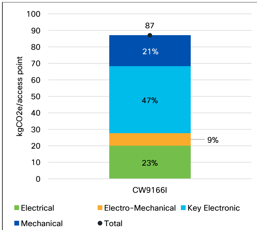
Figure 4: Global Warming Potential per Access Point from Manufacturing Components Across the Upstream Supply Chain
