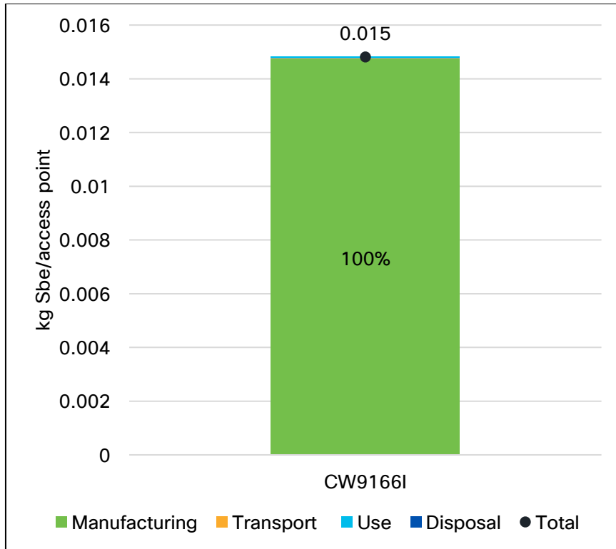
Figure 7: Abiotic Depletion Potential per Access Point by Life Cycle Stage
