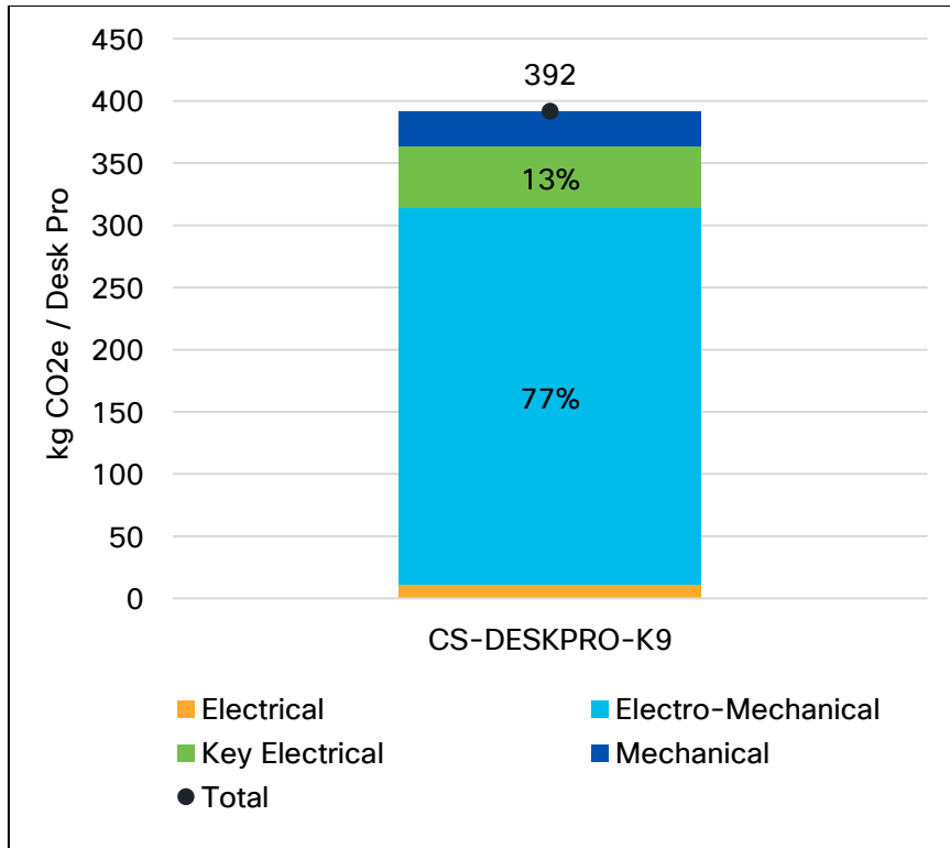
Figure 4: Global Warming Potential per Desk Pro from Manufacturing Components Across the Upstream Supply Chain
