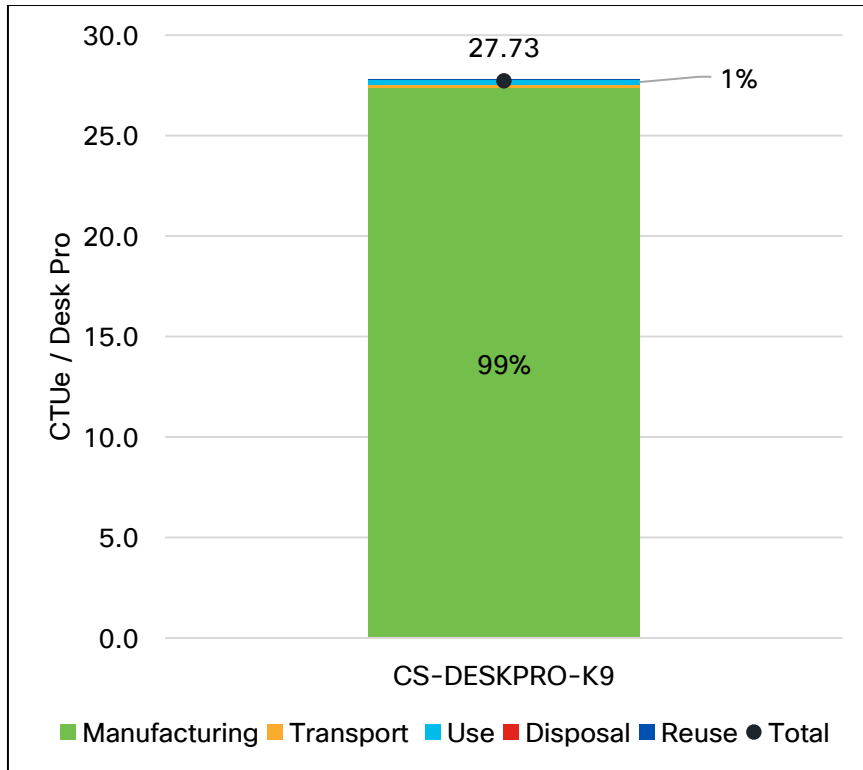
Figure 8: Ecotoxicity per Desk Pro by Life Cycle Stage
