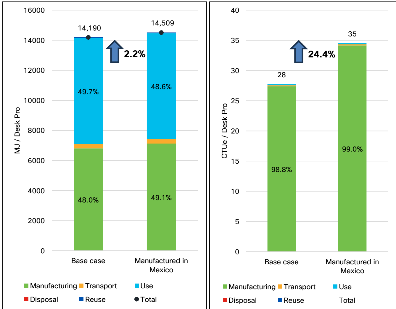
Figure 11: Sensitivity Analysis Results for PED and Ecotoxicity with Desk Pro Manufactured in Mexico
