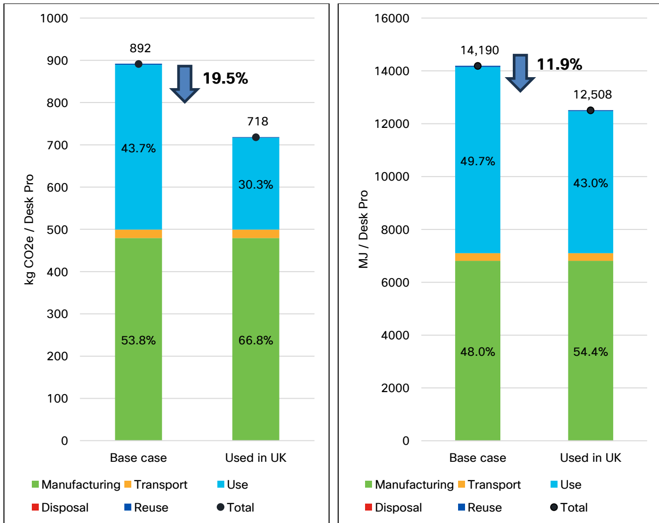
Figure 13: Sensitivity Analysis Results for GWP and PED with Desk Pro Used in the UK
