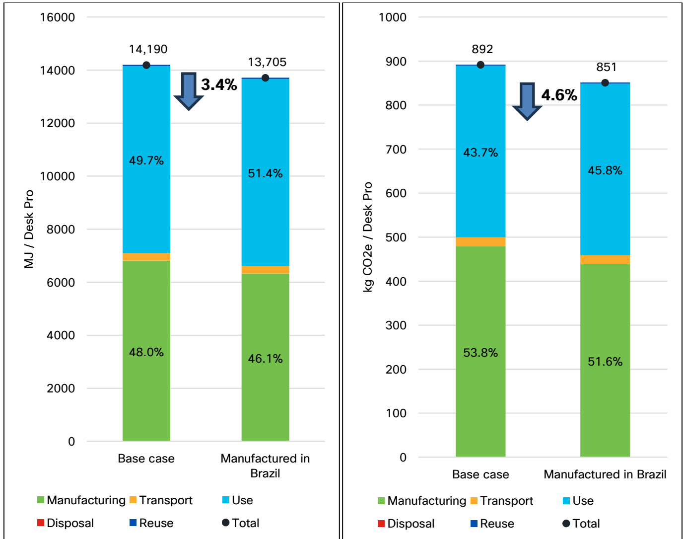
Figure 12: Sensitivity Analysis Results for PED and GWP with Desk Pro Manufactured in Brazil
