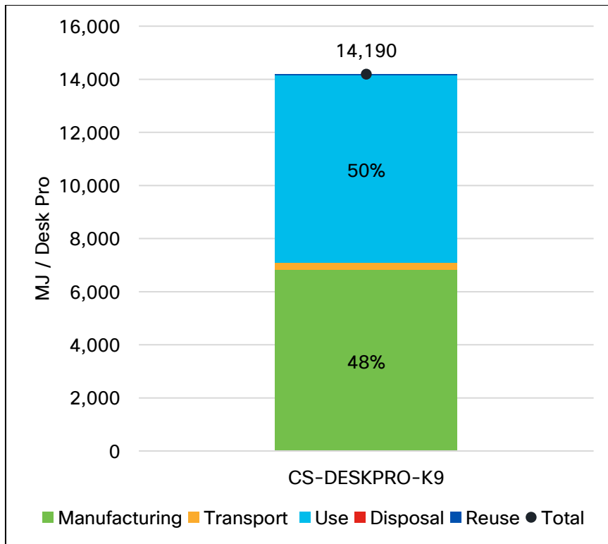
Figure 5: Primary Energy Demand per Desk Pro by Life Cycle Stage
