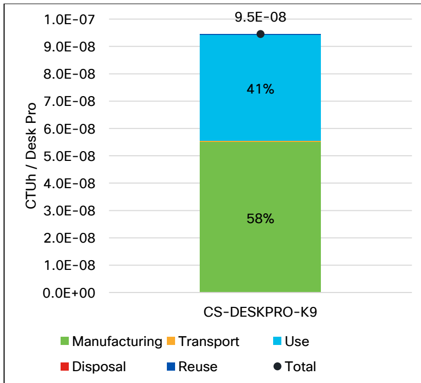
Figure 9: Human Toxicity (Cancer) per Desk Pro by Life Cycle Stage
