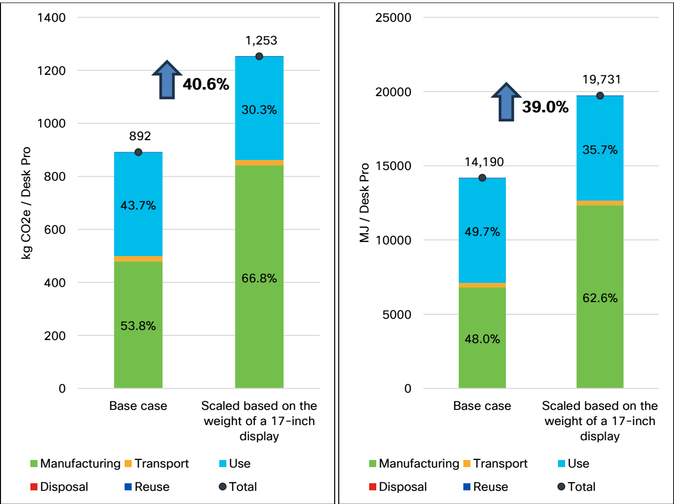
Figure 14: Sensitivity Analysis Results for GWP and PED with Alternative Dataset Used for Display Modeling
