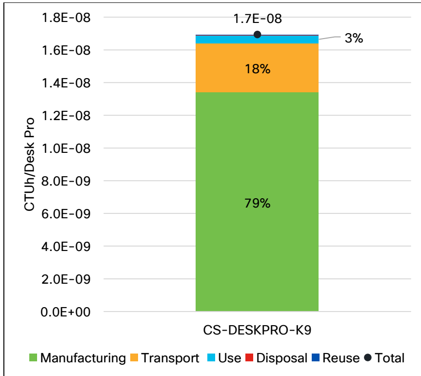
Figure 10: Human Toxicity (Non-Cancer) per Desk Pro by Life Cycle Stage
