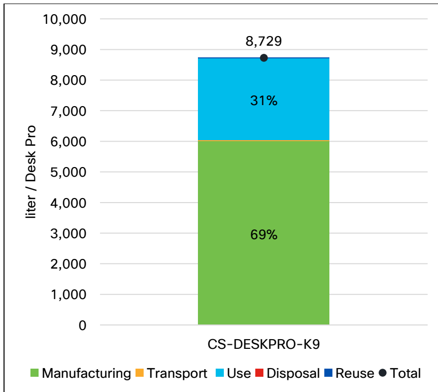
Figure 6: Blue Water Consumption per Desk Pro by Life Cycle Stage
