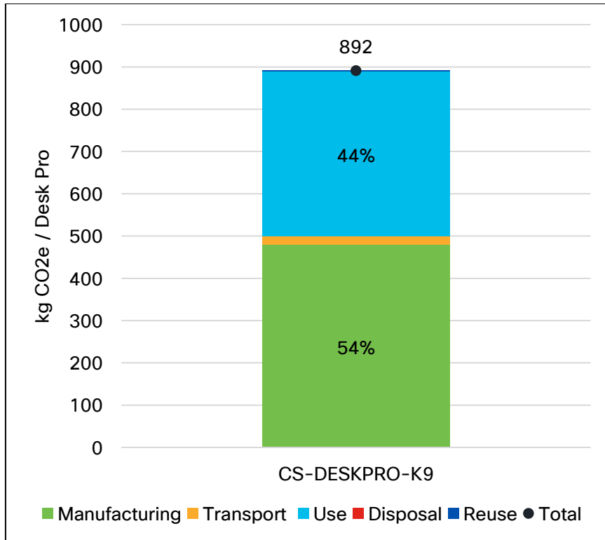
Figure 3: Global Warming Potential Per Desk Pro by Life Cycle Stage
