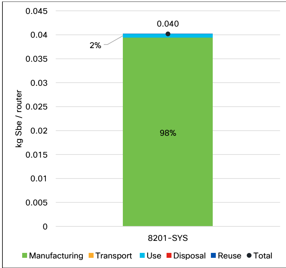
Figure 7: Abiotic Depletion Potential per Router by Life Cycle Stage
