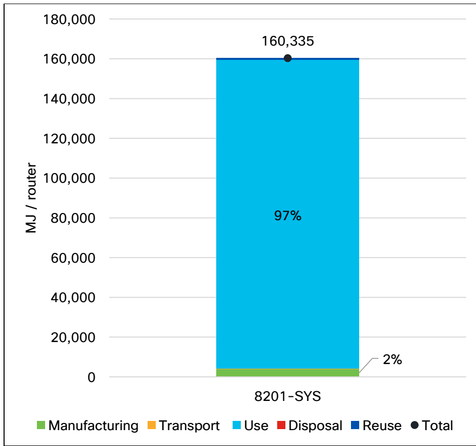
Figure 5: Primary Energy Demand per Router by Life Cycle Stage
