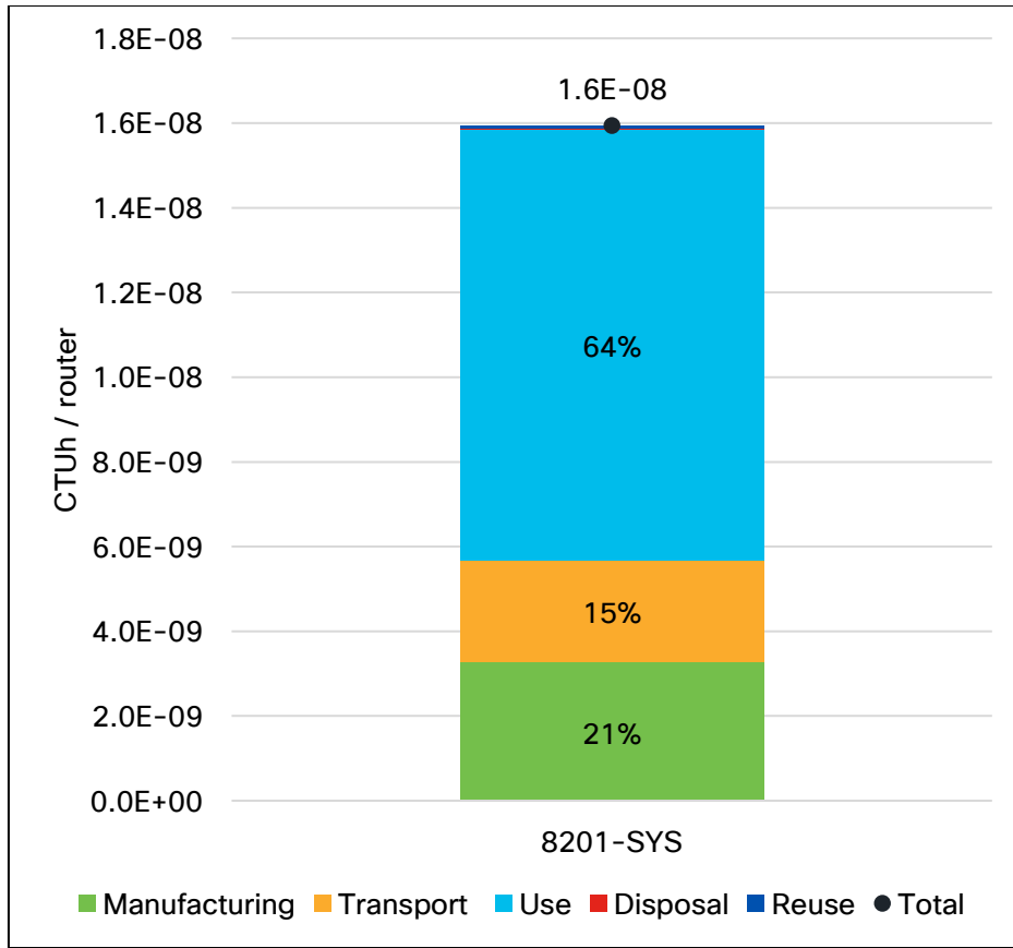
Figure 10: Human Toxicity (Non-Cancer) per Router by Life Cycle Stage
