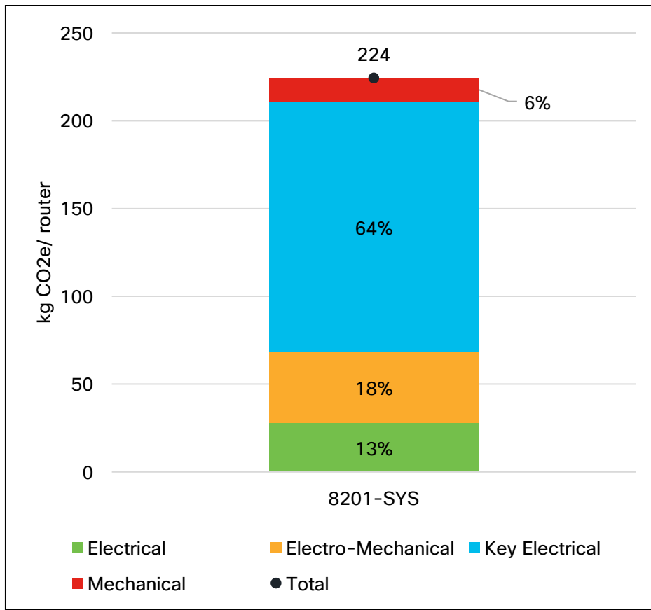
Figure 4: Global Warming Potential per Router from Manufacturing Components Across the Upstream Supply Chain
