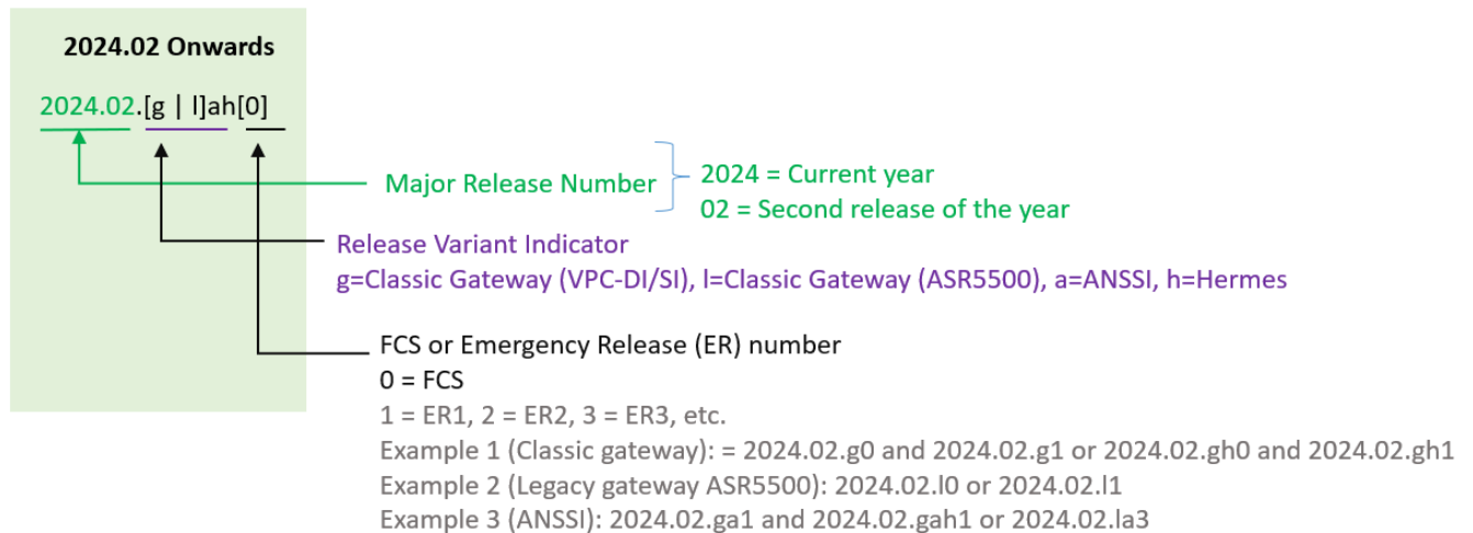
Figure 1 – Version Numbering
