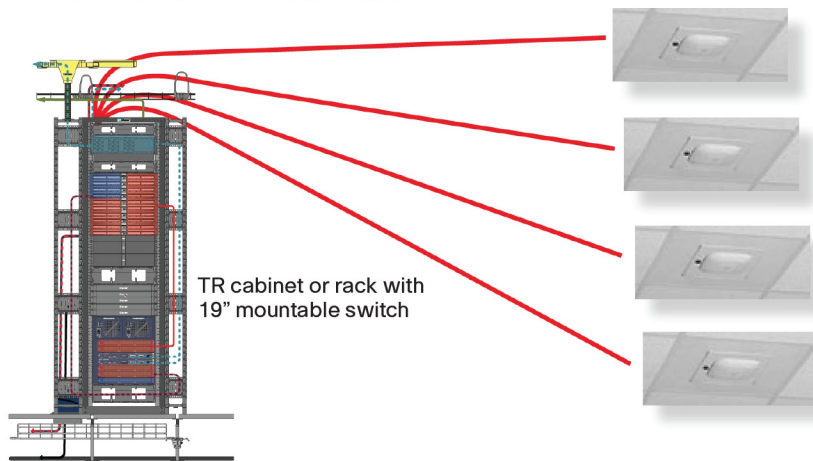
Figure 30 - Wireless access point connections to the TR
