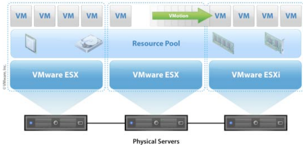
Figure 8) VMware VMotion.
