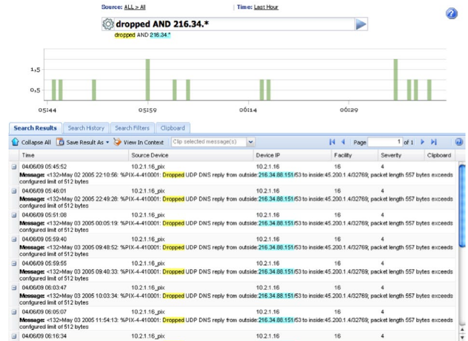
Figure 8 - Index Search Example
