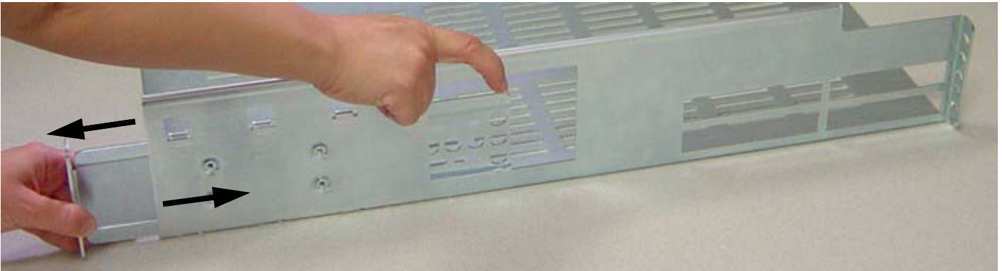
Figure 2-2: Separate the Sliding Bracket From Both Sides of the Shelf Unit
