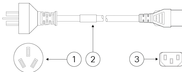
Illustration 12 : Argentine (CAB-ACR)
