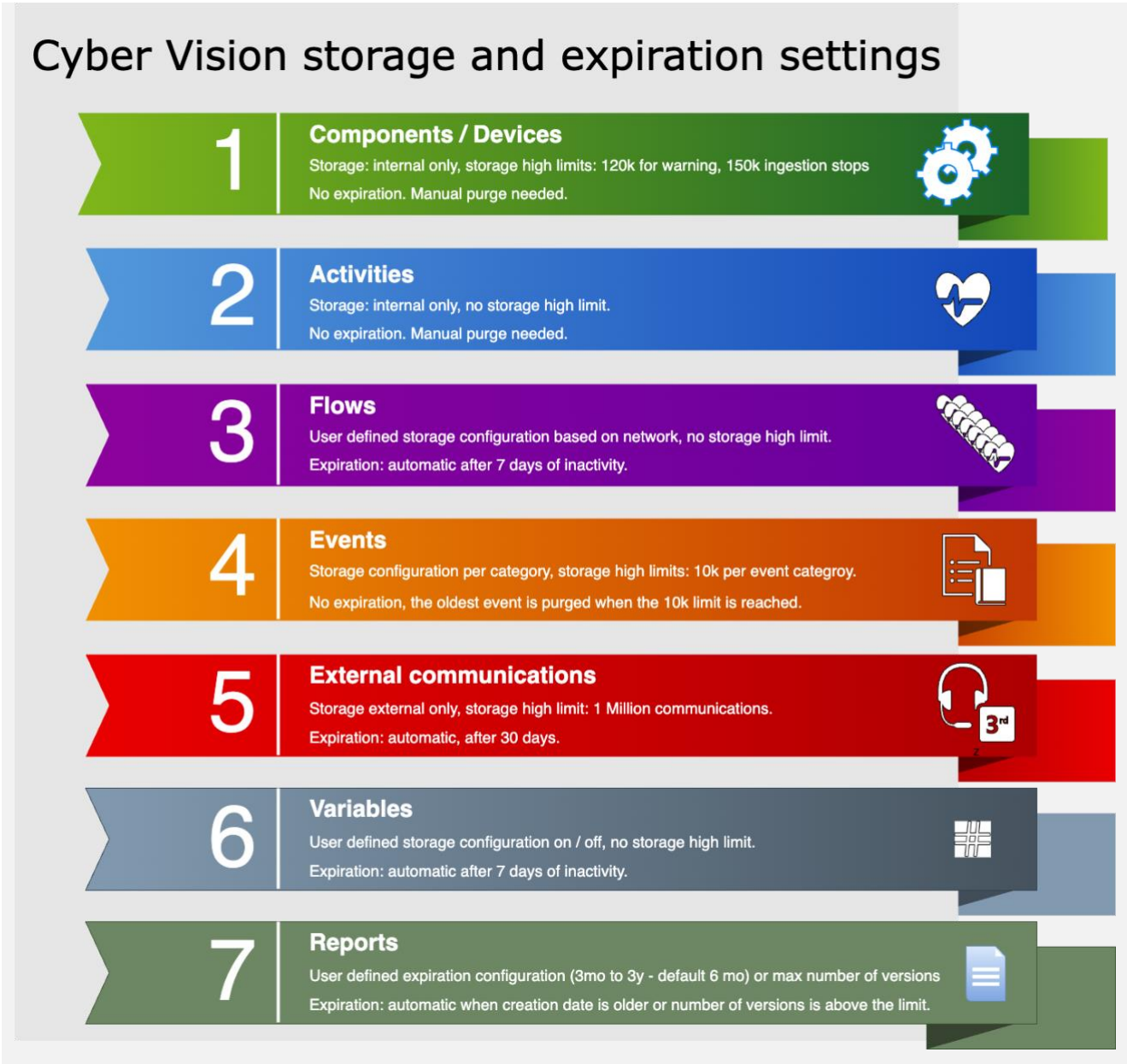
Figure 3. Cisco Cyber Vision data retention policies
