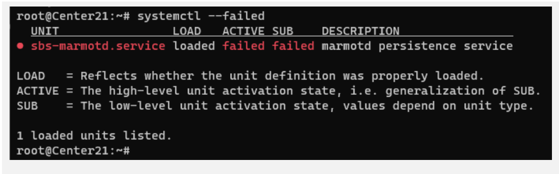
Figure 5. Cisco Cyber Vision system check – example of failure
