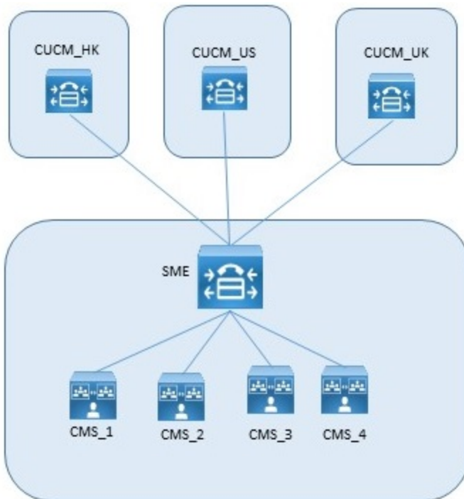
Figure 23: Deployment model with centralized Meeting Servers and an SME to route calls
