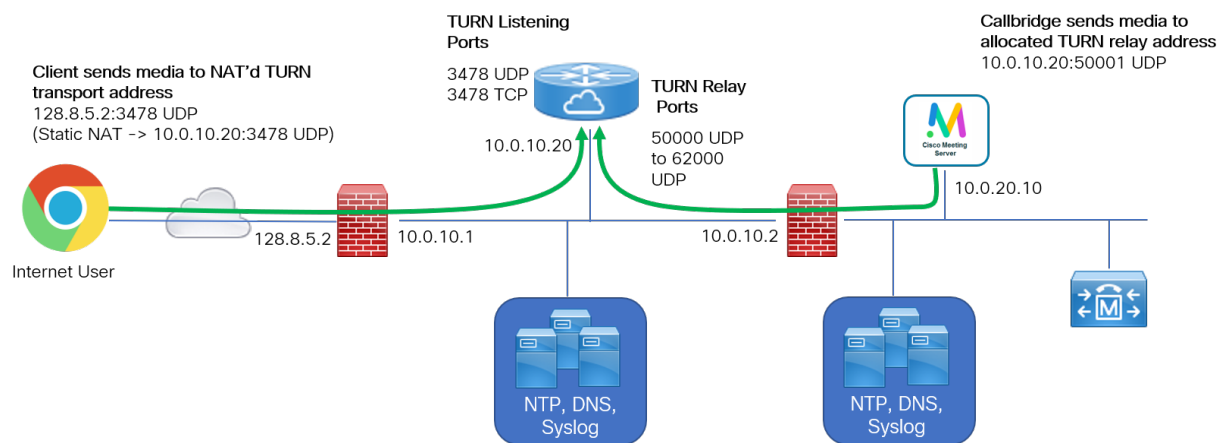
Figure 3: Example of Meeting Server Edge TURN Server
