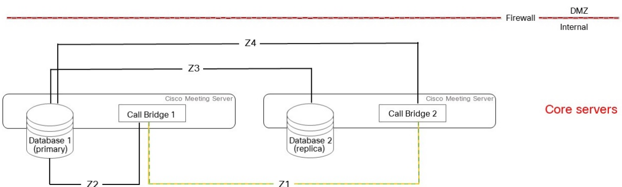
Figure 54: Additional ports required to be open in a scalable and resilient multiple server deployment
