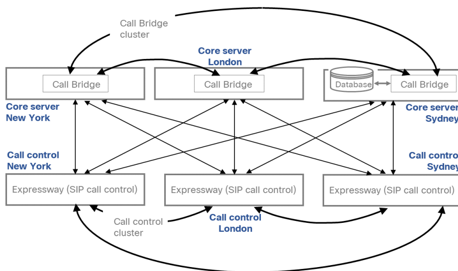
Figure 22: Mesh configuration for SIP Call Control
