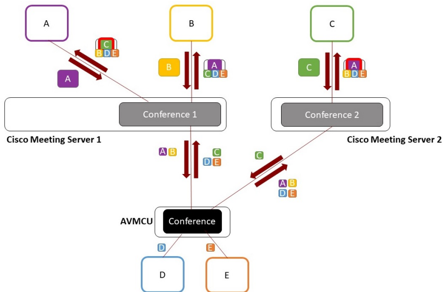
Figure 25: Lync AVMCU/Meeting Server deployment using dualHomeCallBridge mode
