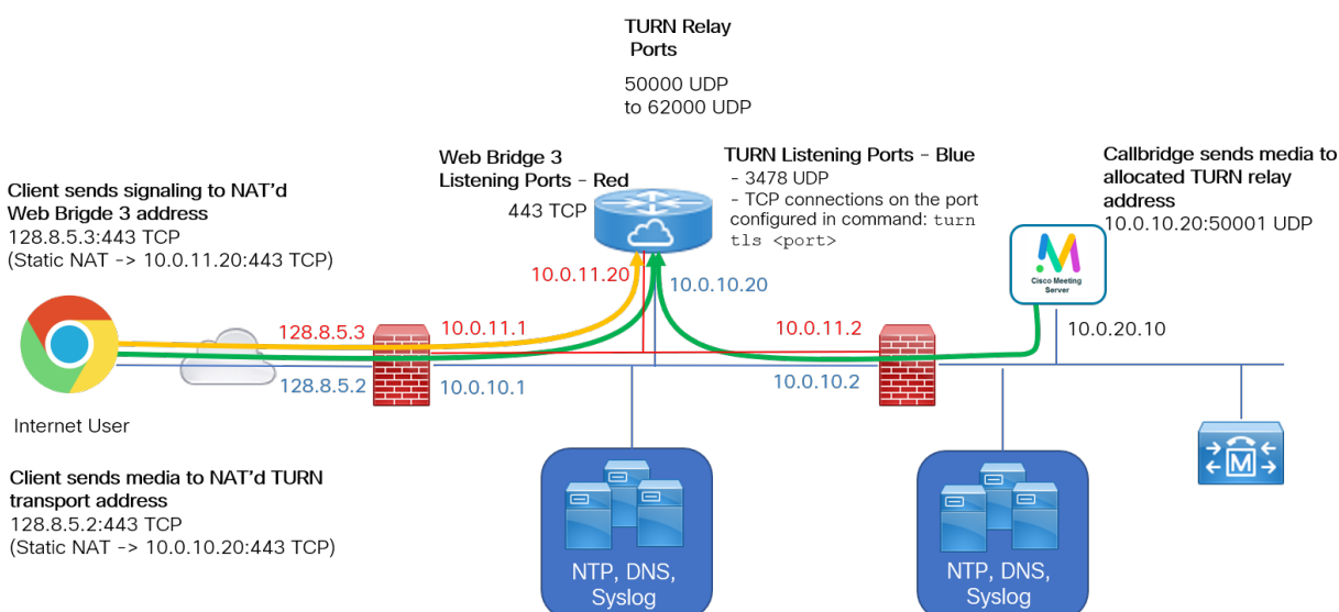
Figure 16: TURN using TCP 443 Example with two interfaces
