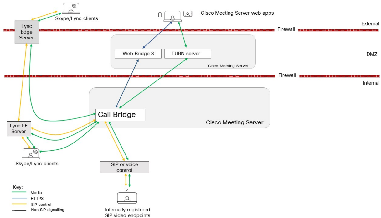
Figure 36: Example Meeting Server deployment for dial plan configuration (using the TURN server component in a split server deployment)
