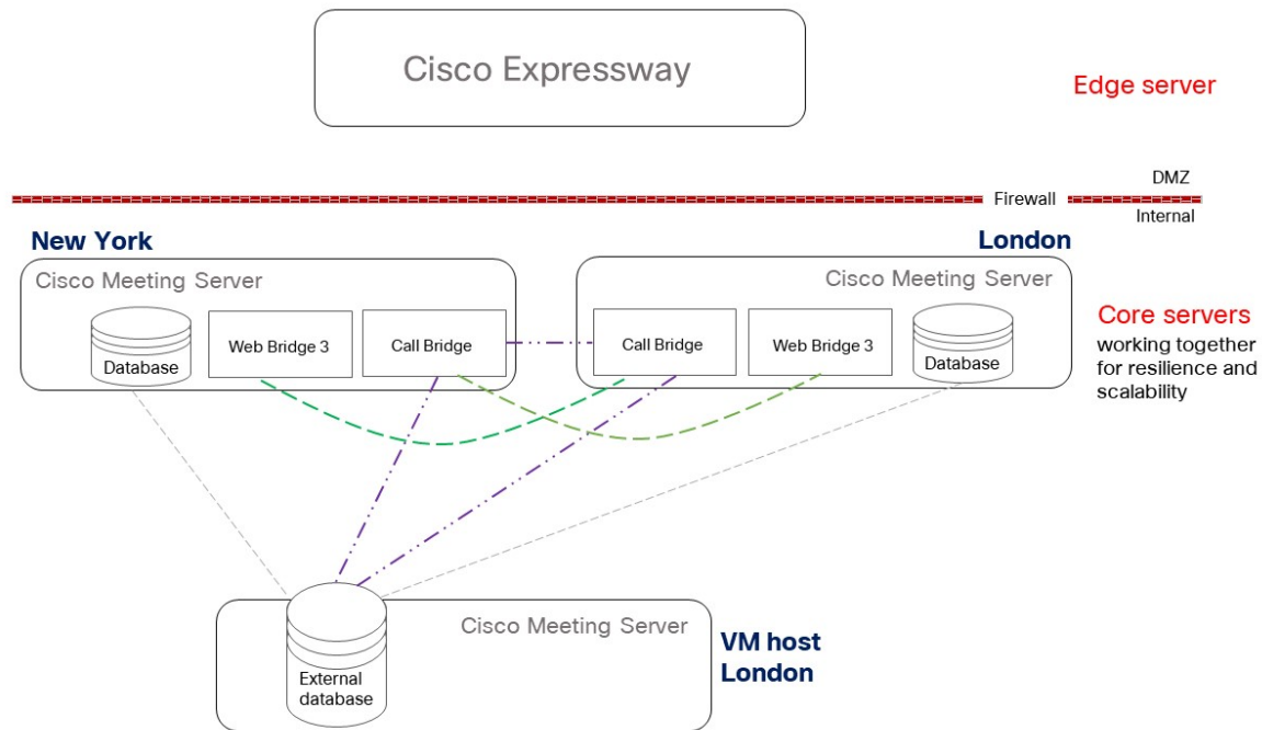
Figure 14: Simple deployment showing connections
