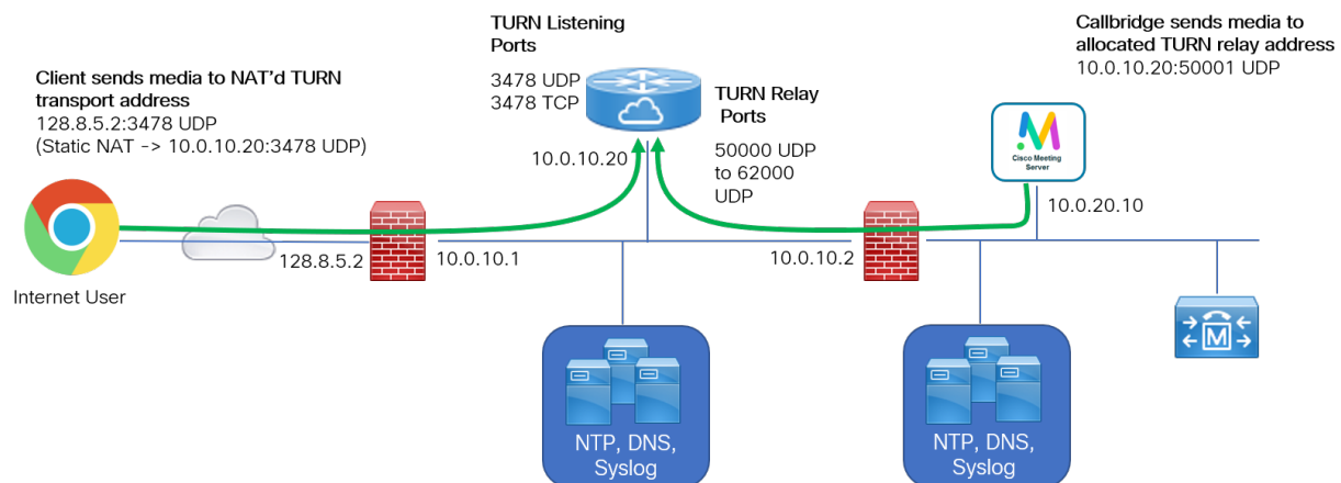
Figure 15: Sample Diagram of TURN using UDP
