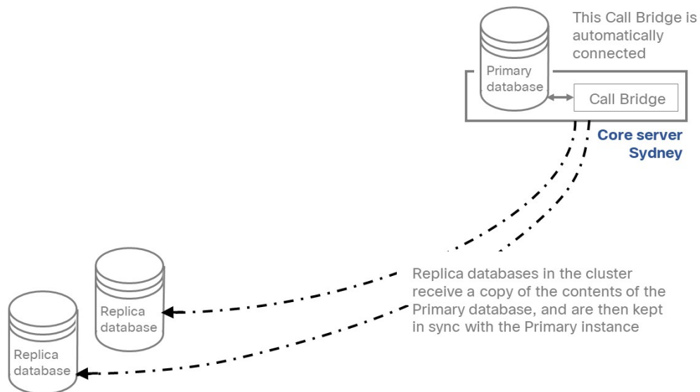
Figure 20: Attaching databases
