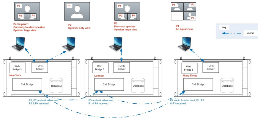
Figure 33: Example media flows and views when PC Clients dial into space A in a combined deployment
