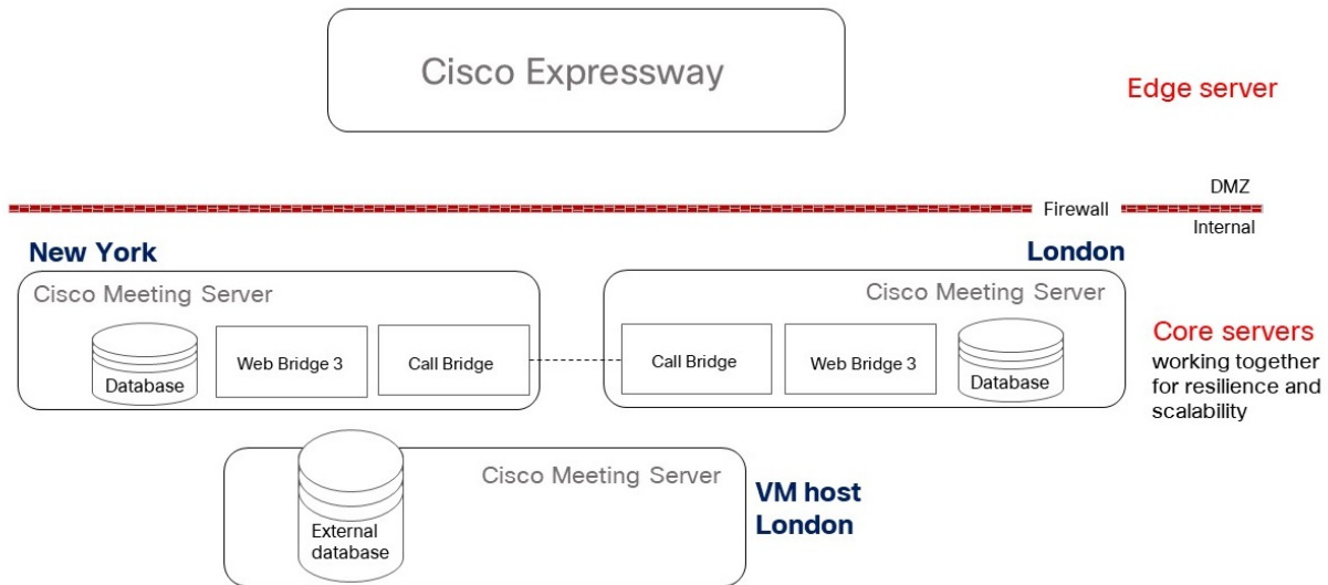
Figure 13: Simplest scaled and resilient configuration
