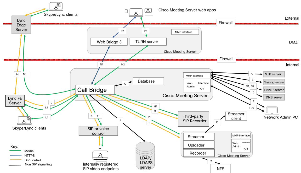
Figure 53: Ports that must be open in a scalable and resilient server deployment using the TURN server and Web Bridge 3 components in the DMZ
