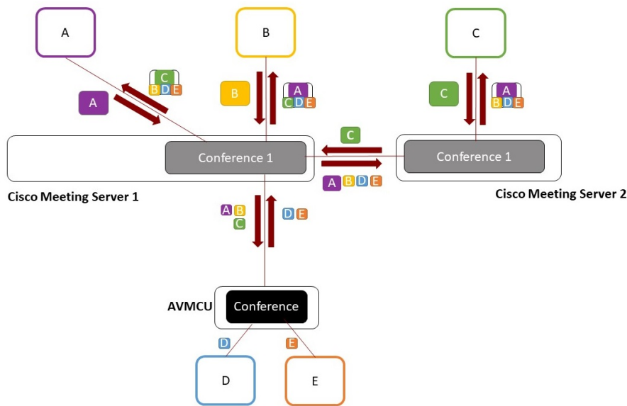
Figure 24: Lync AVMCU/Meeting Server deployment using dualHomeCluster mode
