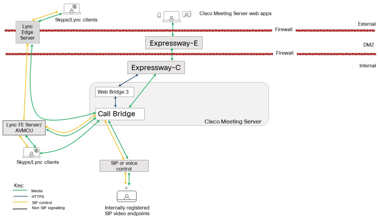
Figure 35: Example Meeting Server deployment for dial plan configuration (with Cisco Expressway at the edge)
