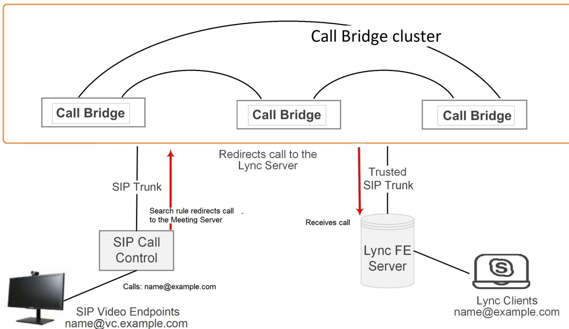
Figure 40: Example of SIP video endpoints and Lync clients in calls
