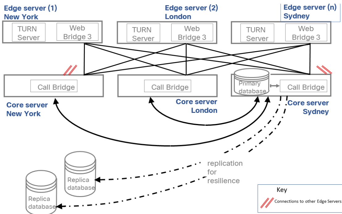
Figure 27: Web Bridges configured in a split deployment
