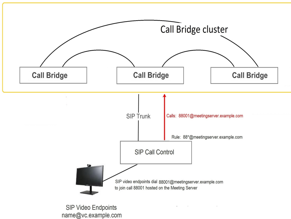
Figure 35: Example of SIP video endpoints calling into clustered Meeting Server hosted calls
