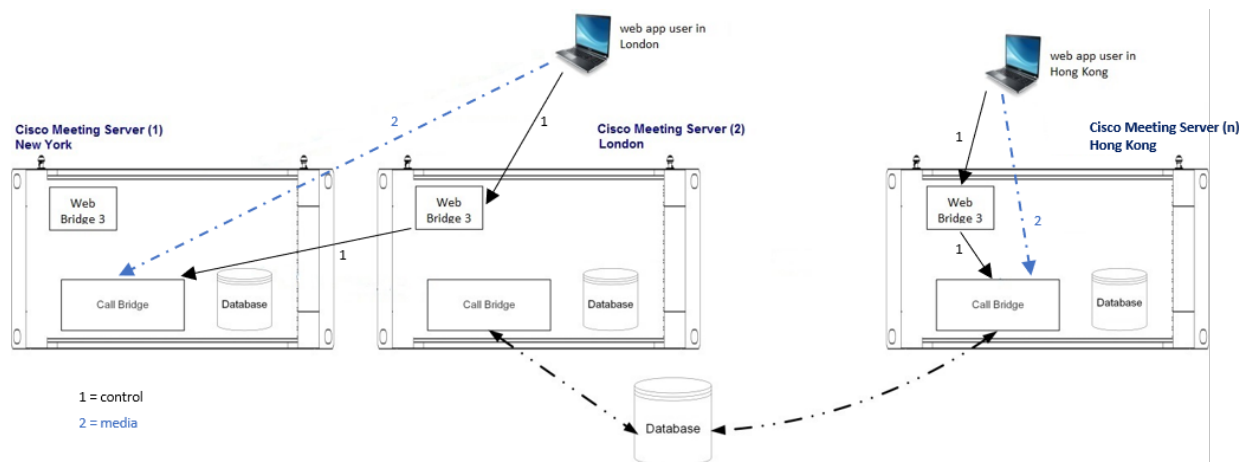
Figure 27: Two web app users making calls to different spaces in a combined deployment
