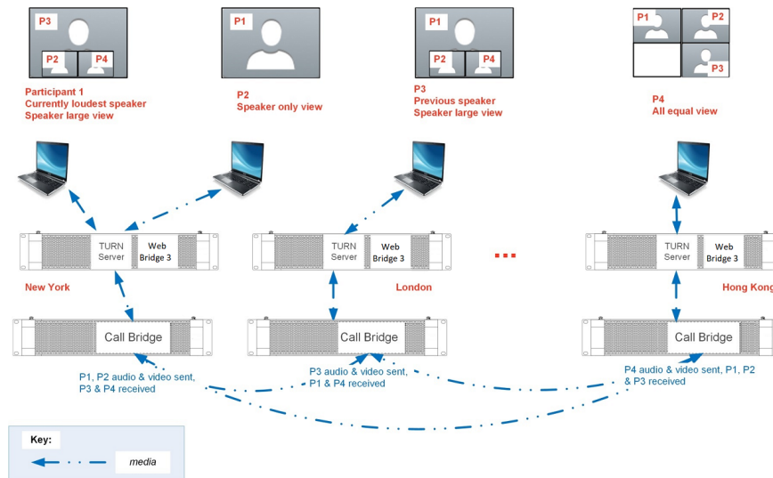
Figure 32: Example media flows and views when PC Clients dial into space A in a split deployment
