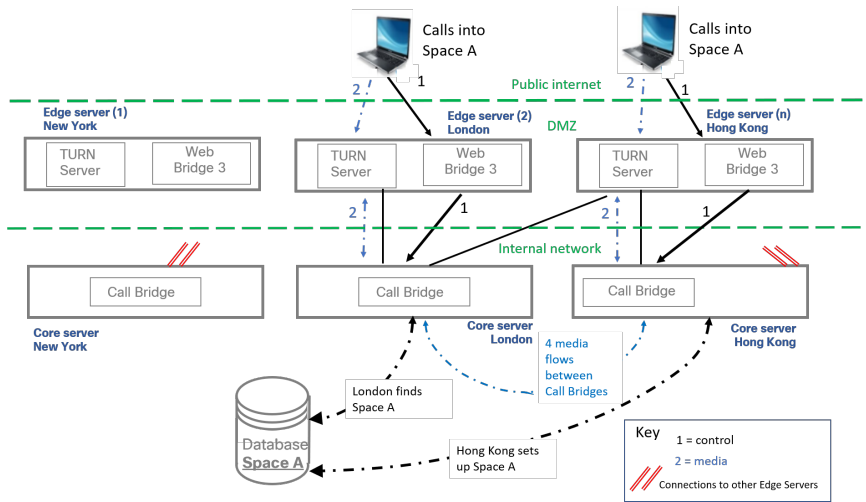
Figure 30: Two Call Bridges calling space A in a split deployment
