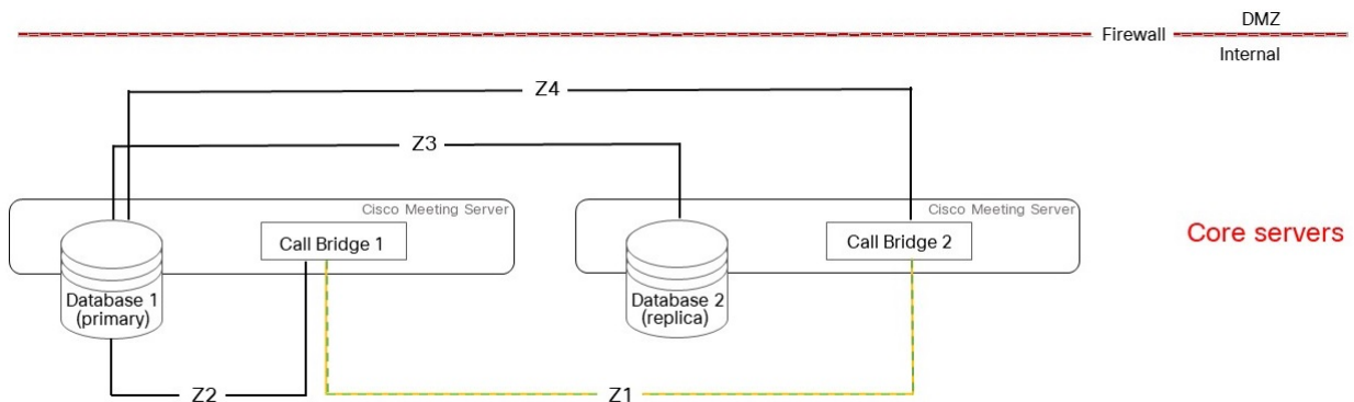
Figure 52: Additional ports required to be open in a scalable and resilient multiple server deployment
