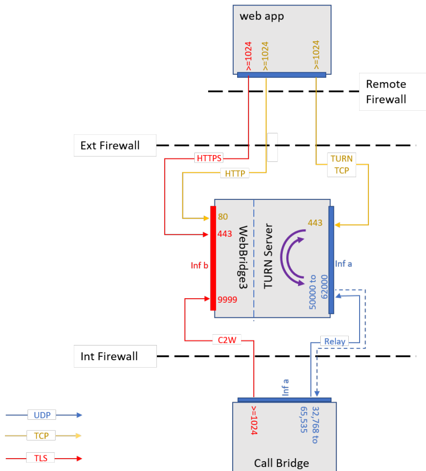
Figure 16: web app using TURN TCP 443 and multiple IPs
