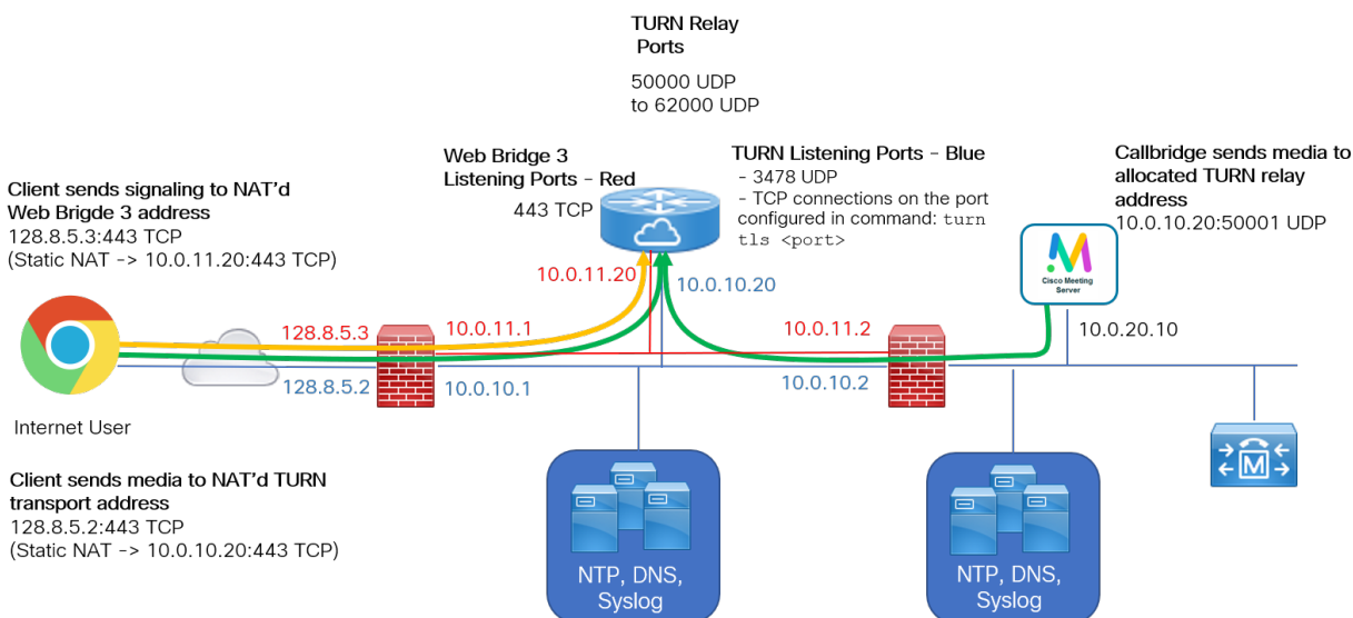
Figure 14: TURN using TCP 443 Example with two interfaces
