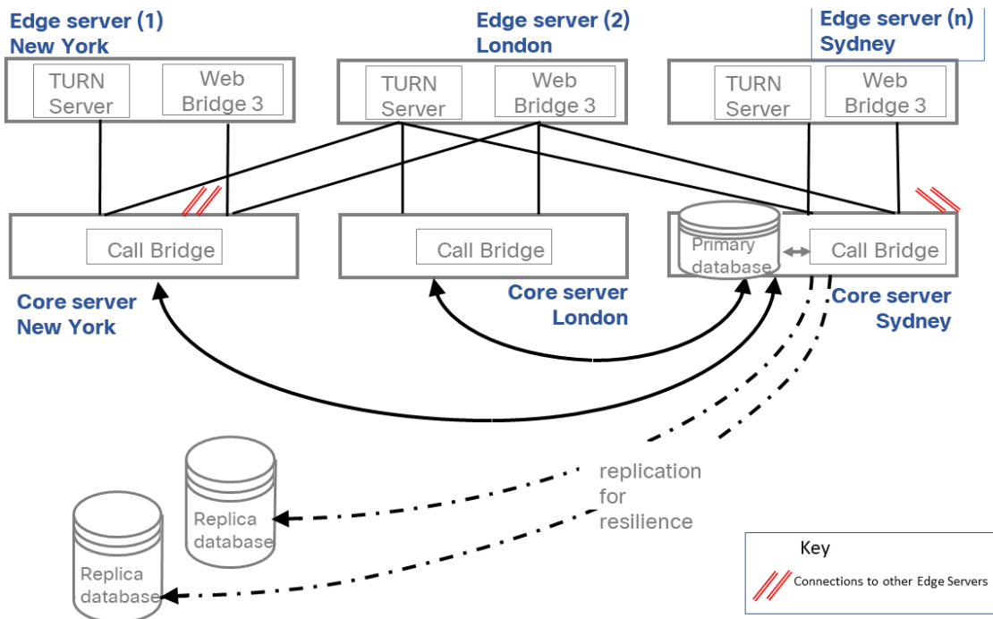
Figure 26: TURN servers configured in a split deployment
