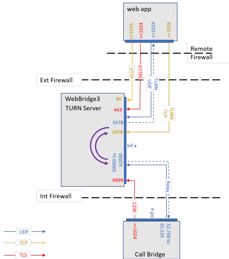
Figure 15: web app using TURN 3478 UDP or 3478 TCP
