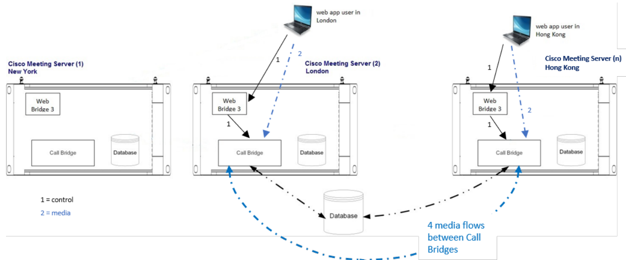
Figure 29: Two Call Bridges calling space A in a combined deployment
