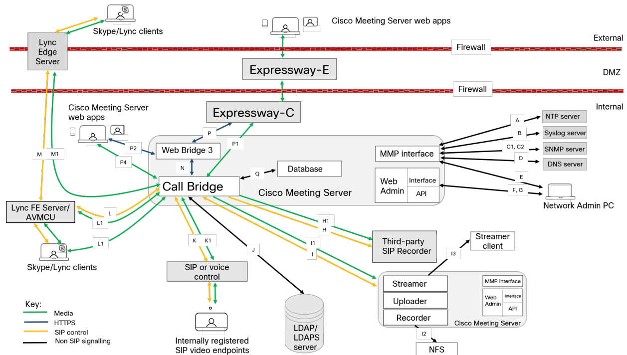
Figure 50: Ports that must be open in a scalable and resilient server deployment with Expressway in the DMZ
