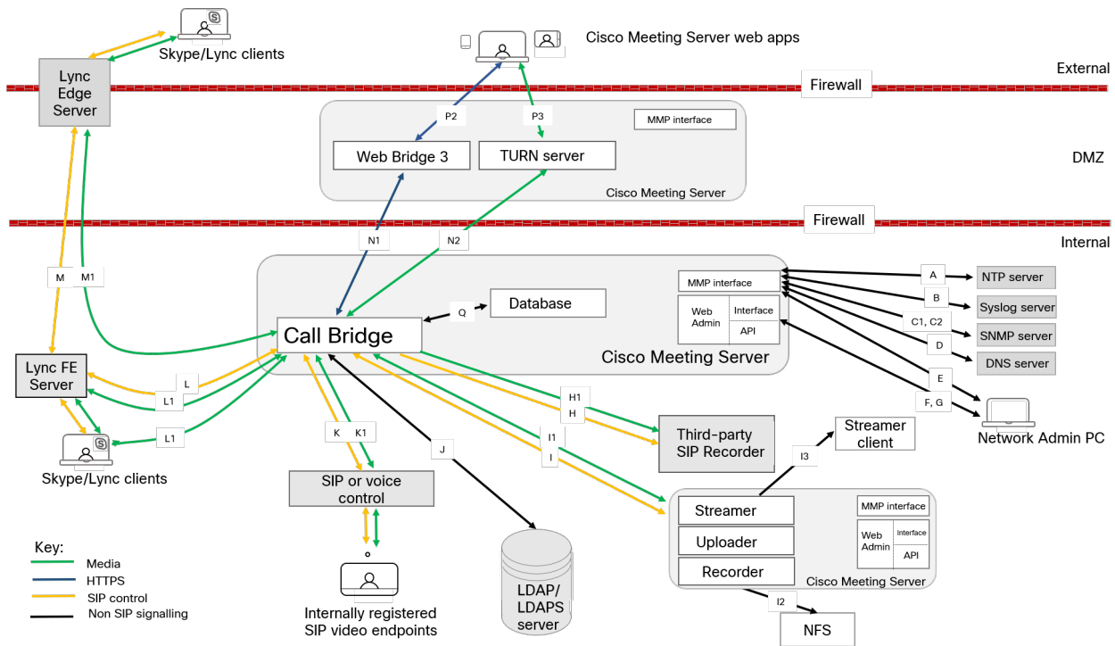
Figure 51: Ports that must be open in a scalable and resilient server deployment using the TURN server and Web Bridge 3 components in the DMZ
