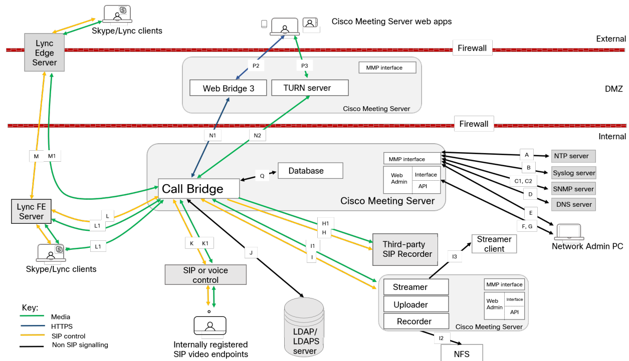
Figure 26: Ports that must be open in a split server deployment using the TURN server and Web Bridge 3 components in the DMZ
