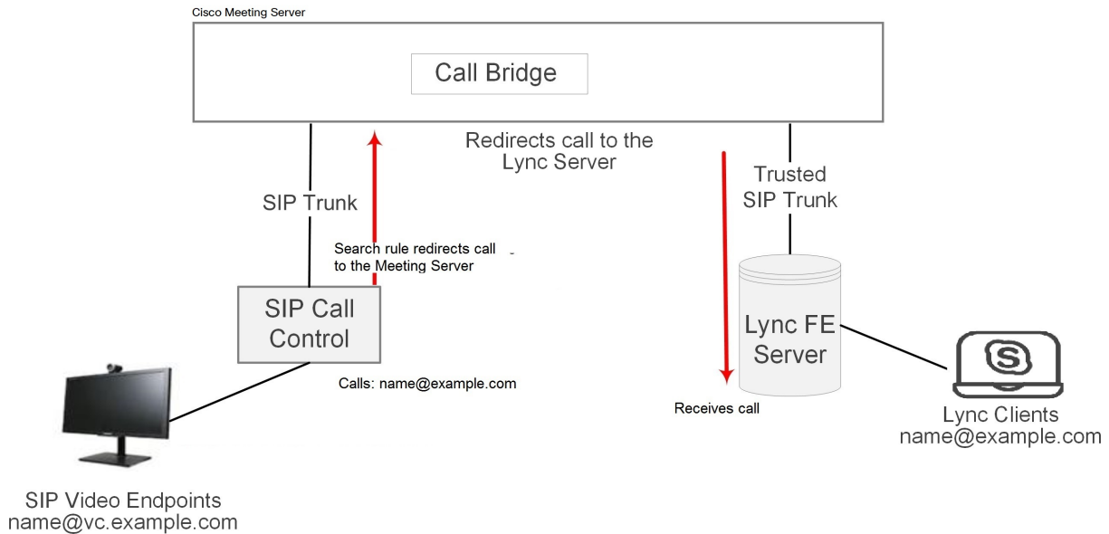
Figure 19: Example of SIP video endpoints and Lync clients in calls
