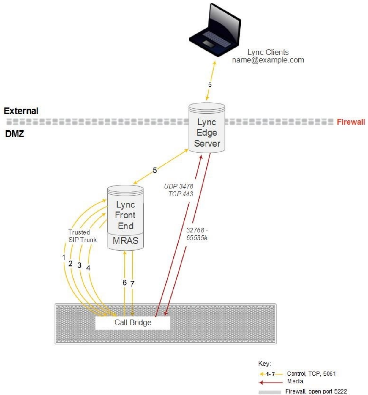
Figure 20: Call Bridge to Lync Edge server call flow
