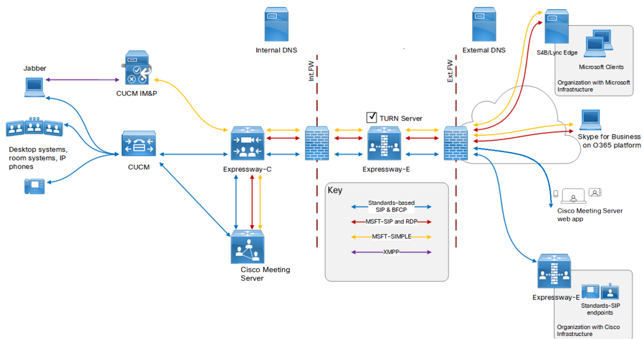
Figure 3: Cisco Unified Communications Manager-centric deployment example
