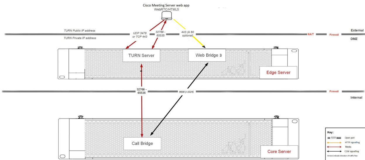
Figure 22: web app port usage
