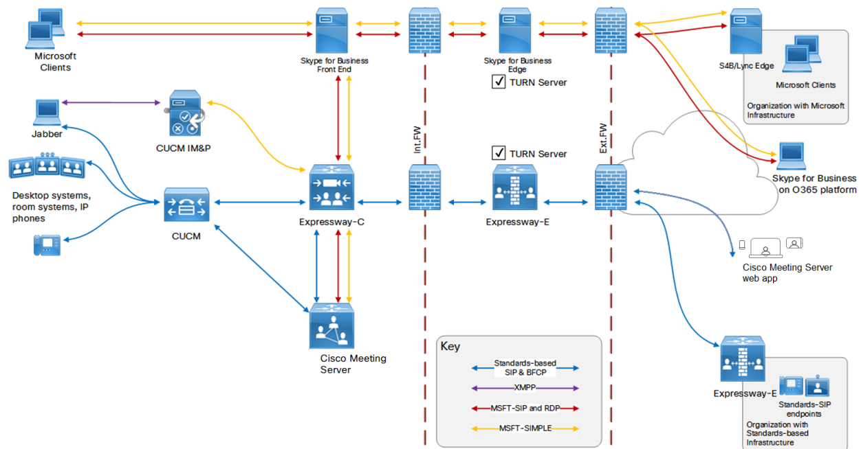
Figure 4: Cisco and Microsoft Infrastructure on-premises deployment example
