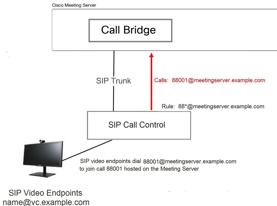
Figure 16: Example of SIP video endpoints calling into Meeting Server hosted calls
