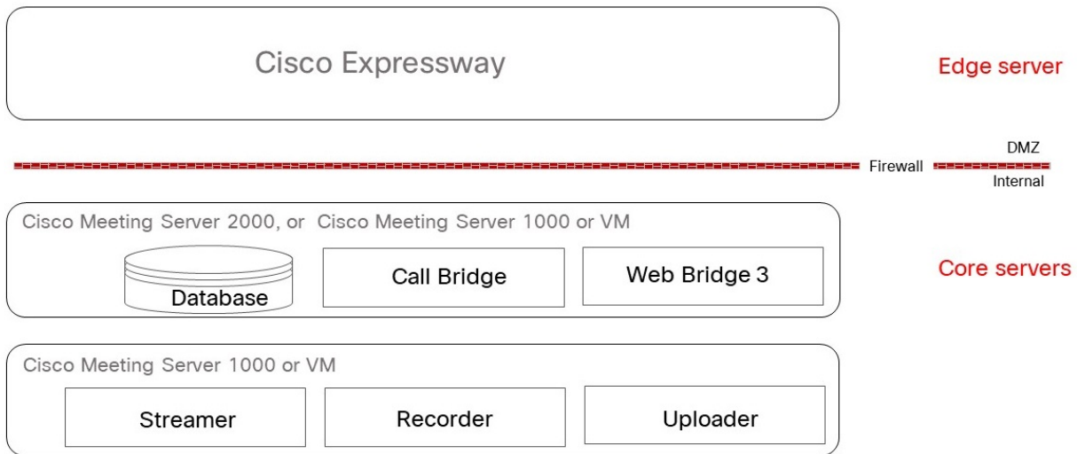
Figure 1: Split server deployment with Cisco Expressway providing TURN services
