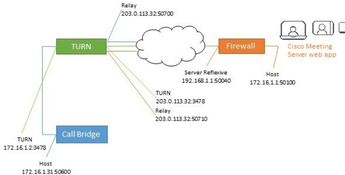
Figure 35: Split Meeting Server deployment with external web app users (no NAT)
