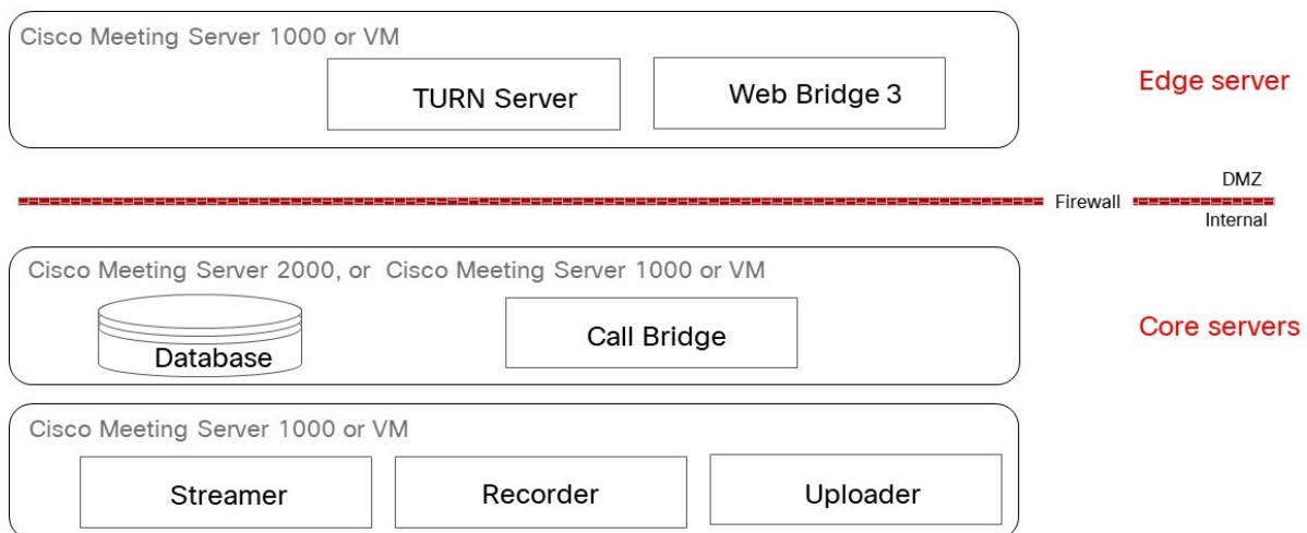
Figure 2: Split server deployment with Cisco Meeting Server providing TURN services
