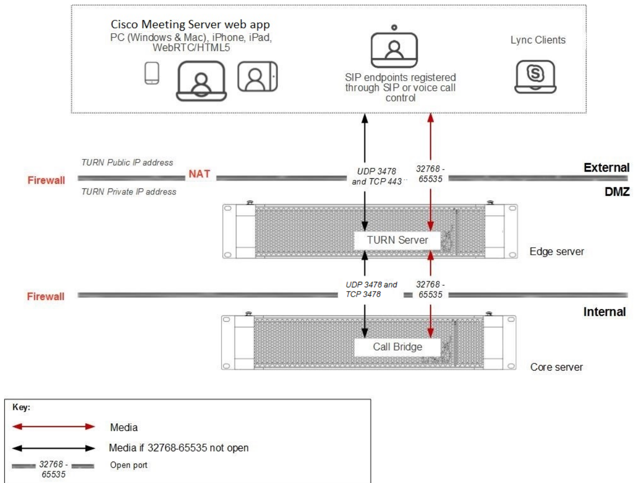
Figure 21: Ports used by TURN Server
