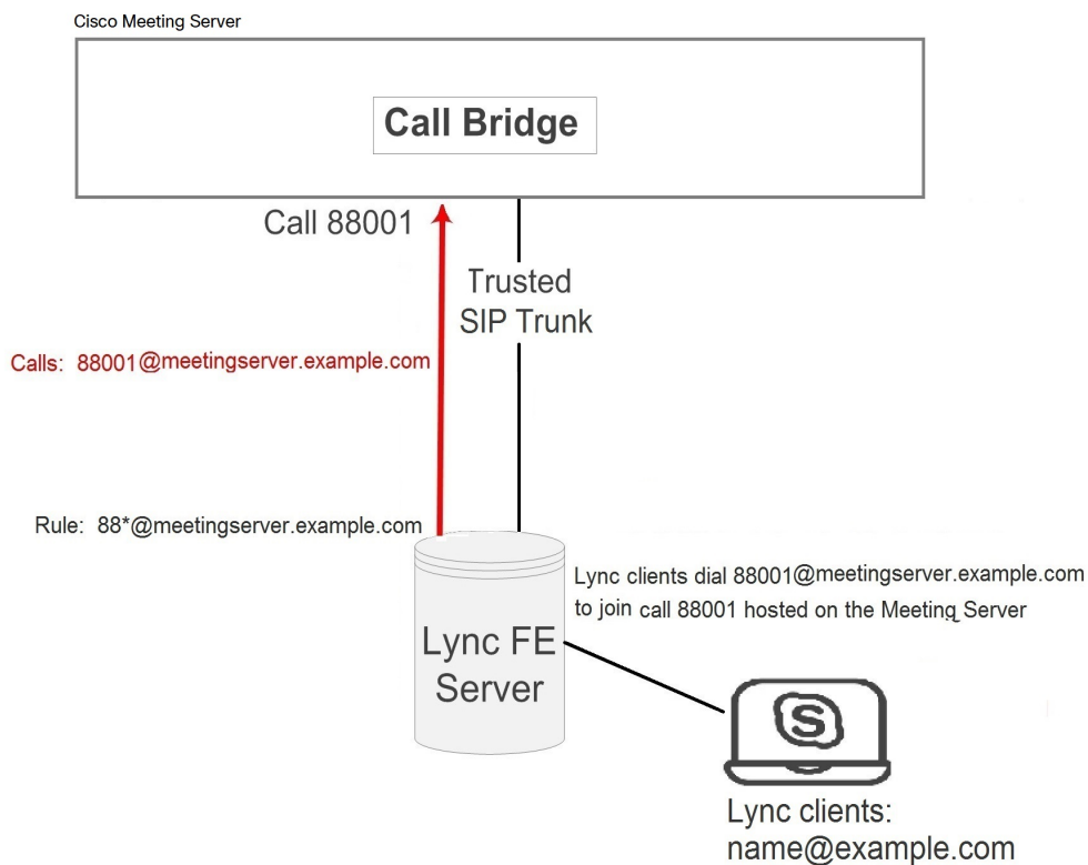
Figure 17: Example Lync clients calling into Meeting Server hosted meetings
