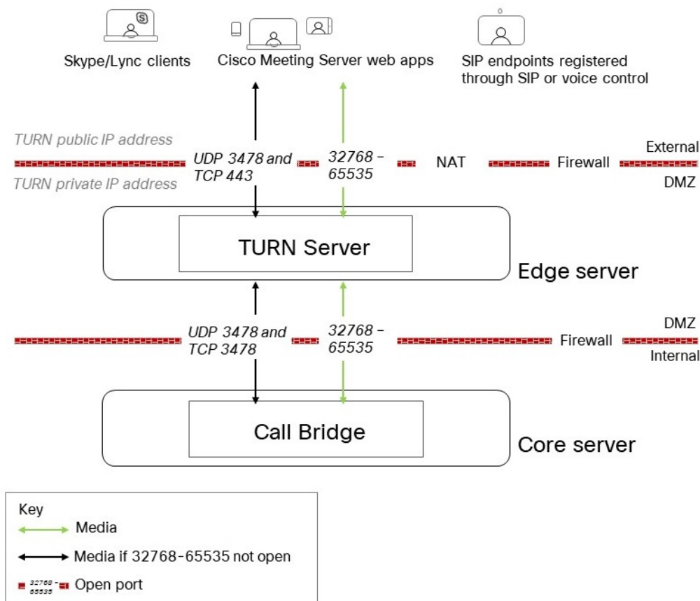
Figure 14: TURN server public IP address (not NAT'ed) – Split server deployment
