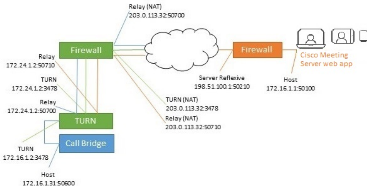
Figure 37: Split Meeting Server deployment with external web app users (with NAT)
