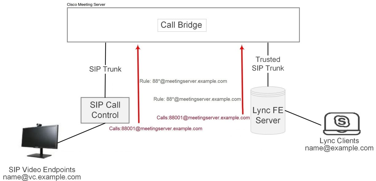
Figure 18: Example of SIP video endpoints and Lync clients calling into Meeting Server hosted meetings
