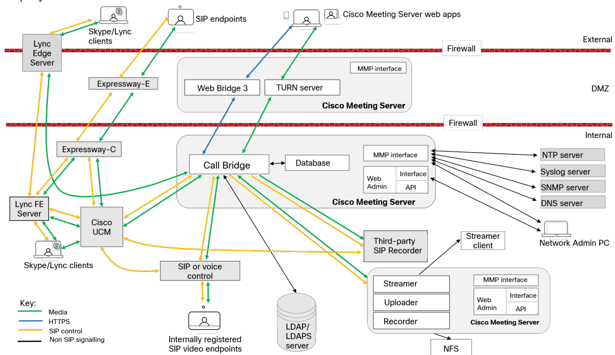
Figure 11: Example of a Meeting Server deployment using the TURN server component in a split server deployment
