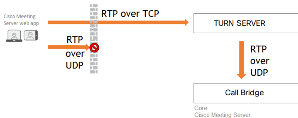
Figure 12: TURN server supporting TCP and UDP
