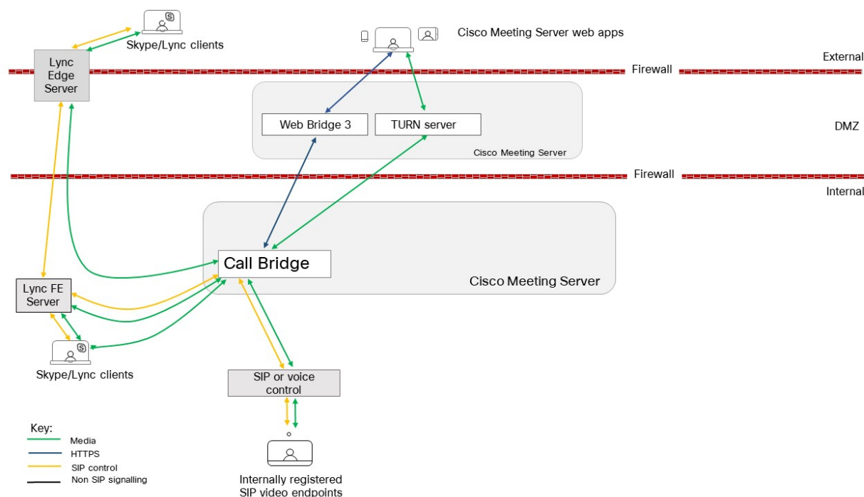
Figure 15: Example deployment for dial plan configuration
