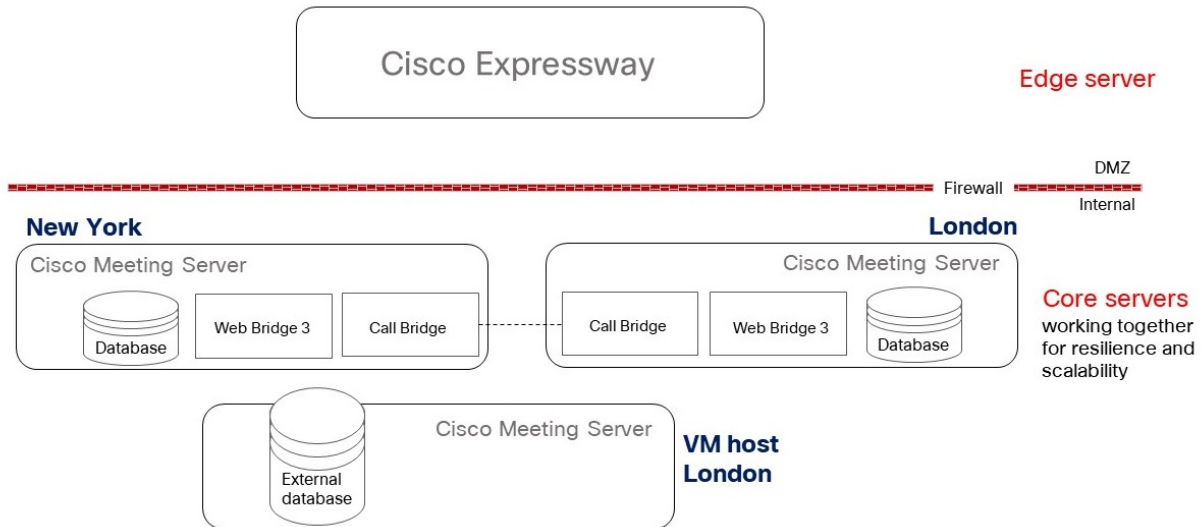
Figure 11: Simplest scaled and resilient configuration
