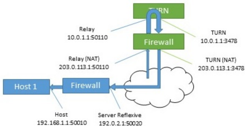
Figure 28: TURN server returns relay address to host
