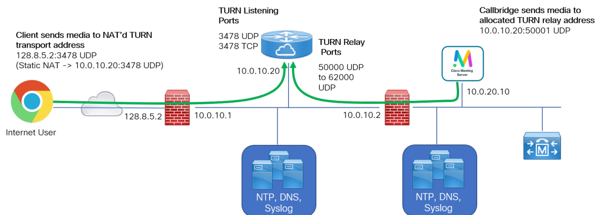
Figure 2: Example of Meeting Server Edge TURN Server
