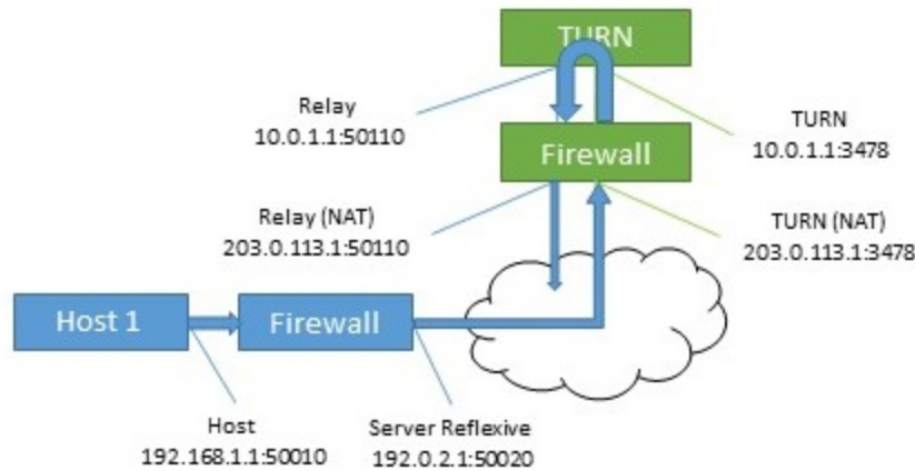
Figure 29: Host sending packets to the far end
