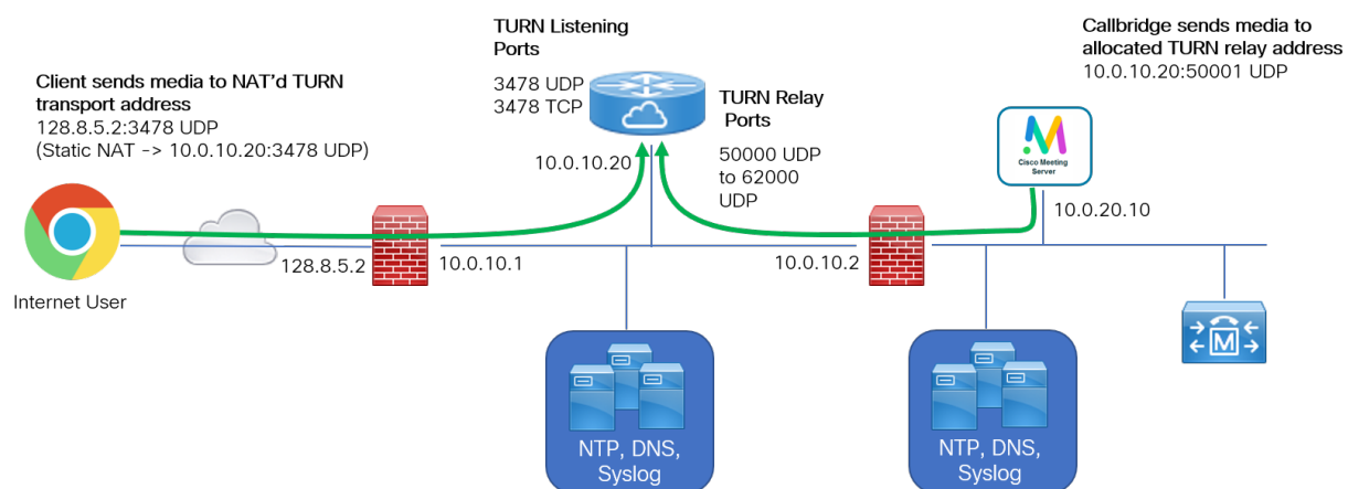
Figure 8: Sample Diagram of TURN using UDP
