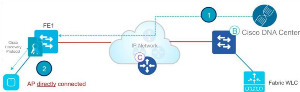
Figure 16. Connecting and discovering the AP
