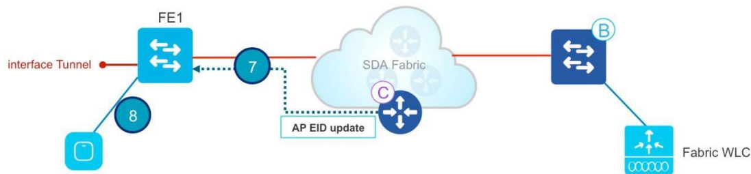
Figure 19. Creating a VXLAN tunnel for the AP
