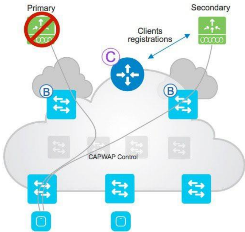
Figure 47. N+1 redundancy
