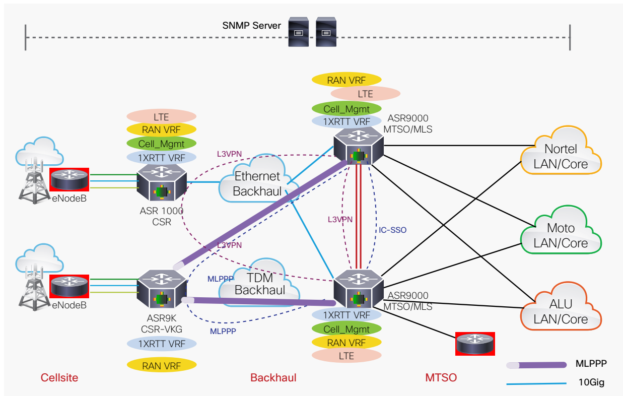
Figure 1. MBH High-Level Topology Overview
