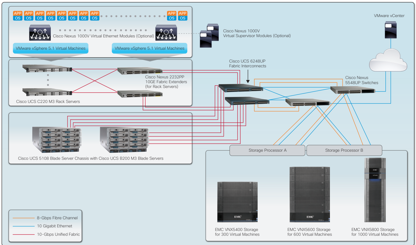
Figure 1. Cisco Virtualization Solution for EMC VSPEX with VMware vSphere 5.1 Configuration
