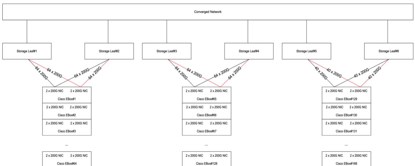
Figure 5: Cisco EBox storage cluster network topology with 128 x 400G switches supporting 16,384 GPUs
