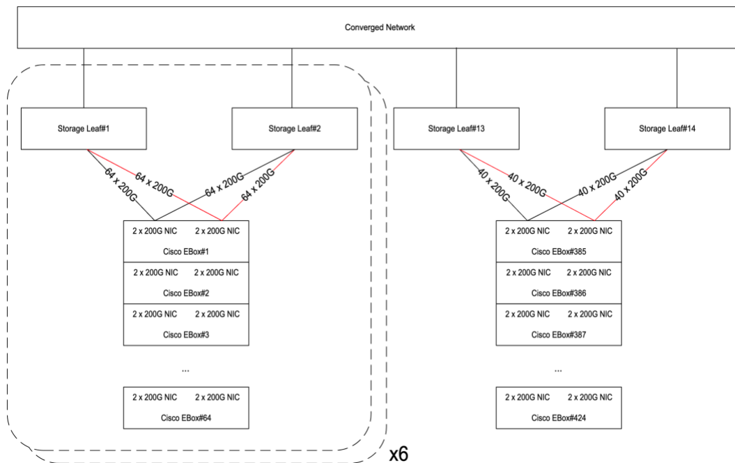
Figure 6: Cisco EBox storage cluster network topology with 128 x 400G switches supporting 41,472 GPUs
