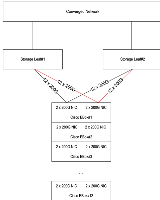
Figure 4: Cisco EBox storage cluster network topology supporting 1024 GPUs
