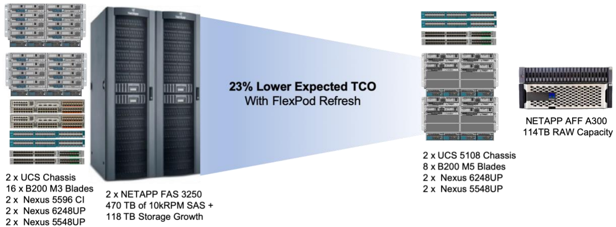
Figure 5. Existing and Proposed Refreshed FlexPod Solution Used in Modeled Scenario
