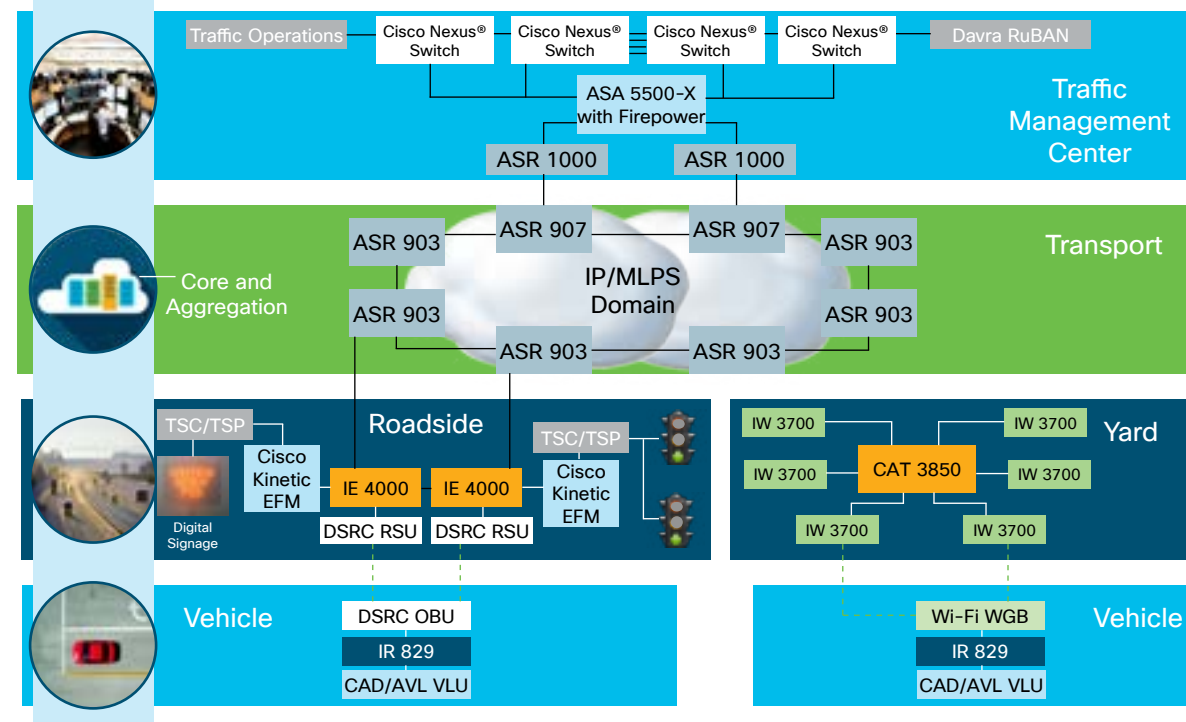
Figure 1. Key elements the Cisco Connected Roadway solution
