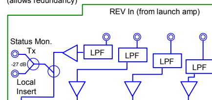
p/n 591158 Quad Segmentation (4X) Reverse Router Module (Four Wide) 5-55 MHz (no redundancy)
