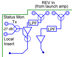
p/n 591165 Dual Segmentation (2X) Reverse Router Module (Two Wide) 5-65 MHz (no redundancy)
