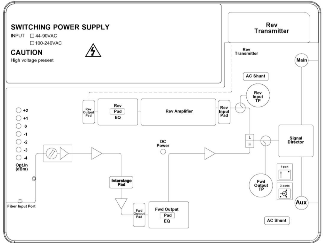
Figure 3. Block Diagram
