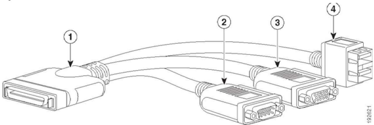
Figure 6 KVM Cable
