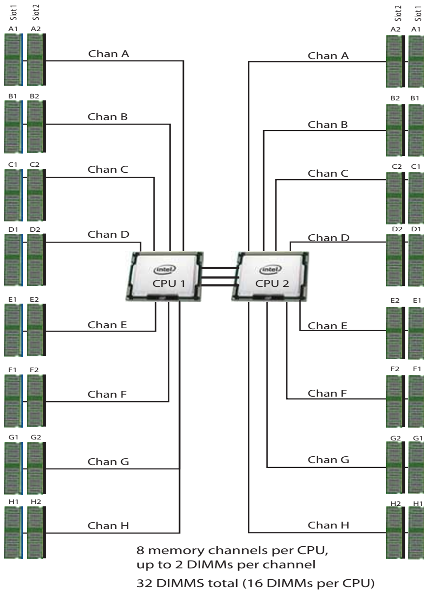
Figure 4 Memory Organization
