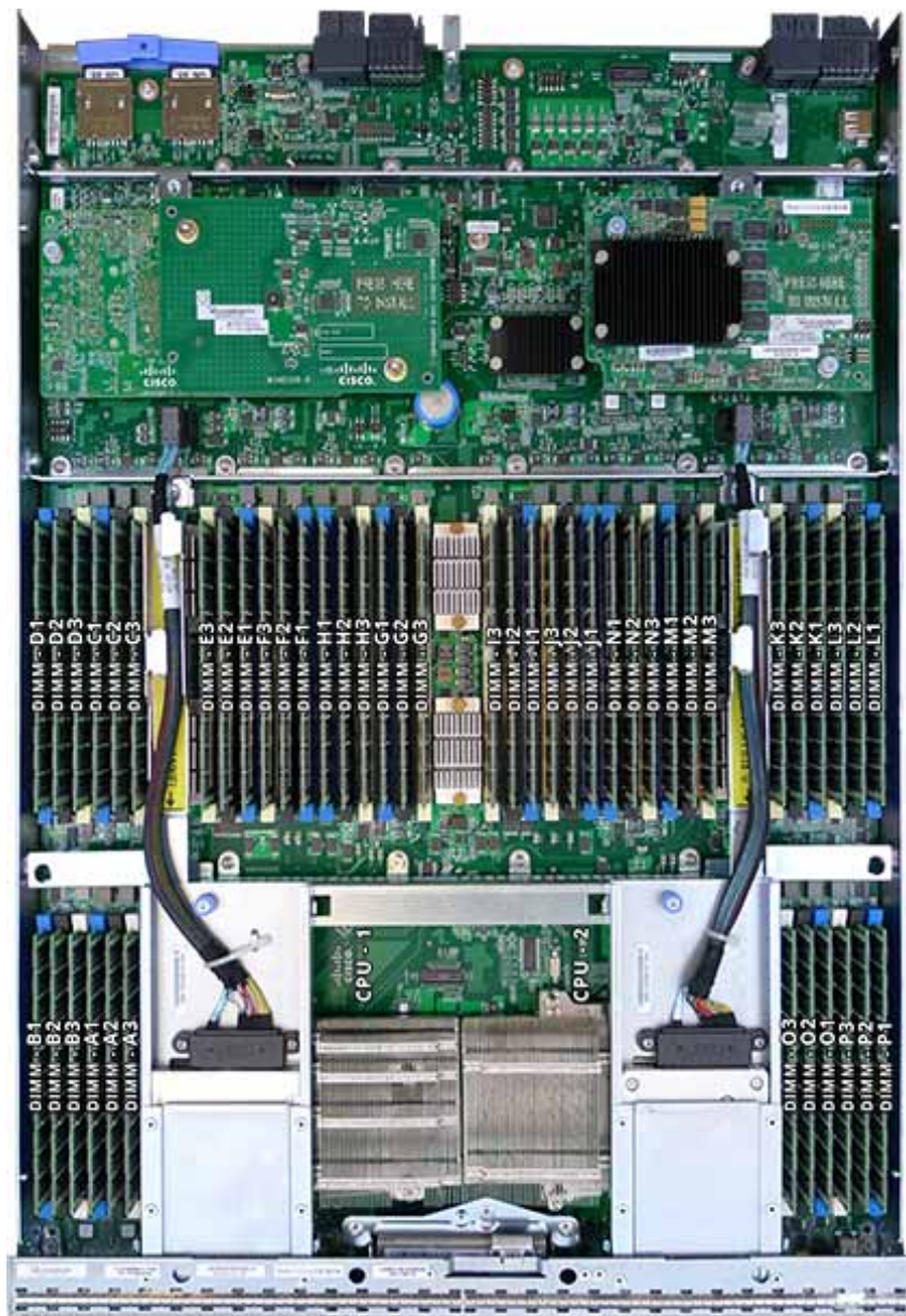
Figure 5 Top view of one of the two Blade Modules for B460 M4 E7 v4 (cover off)
