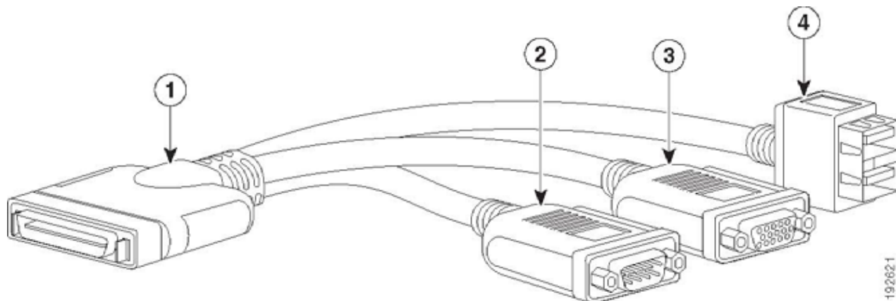
Figure 4 KVM Cable
