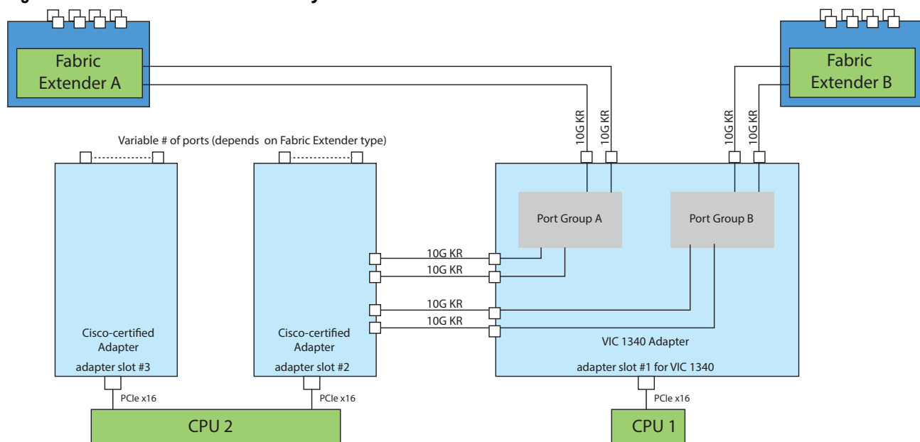
Figure 9 VIC 1340 Connectivity
