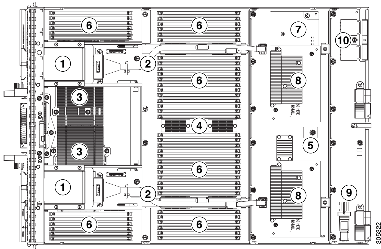
Figure 6 B260 M4 E7 v4 Top View (cover off)
