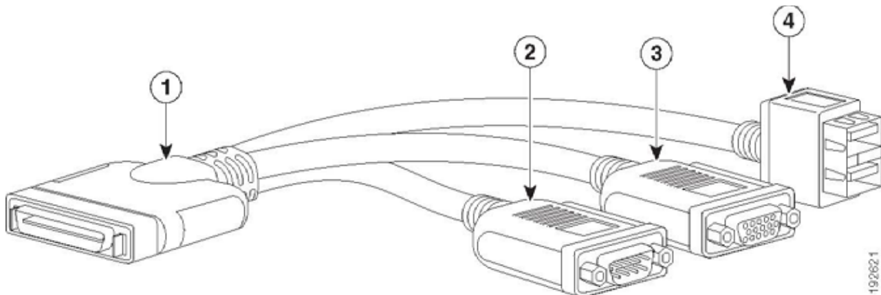
Figure 4 KVM Cable
