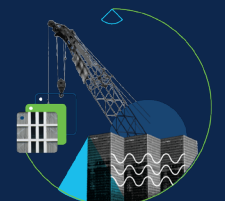
Application Security
