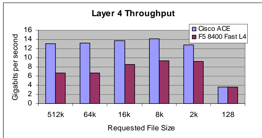
Chart 1: Results of Layer 4 Throughput for Cisco ACE and F5 BIG-IP 8400 w/ F5 FastL4 profile
