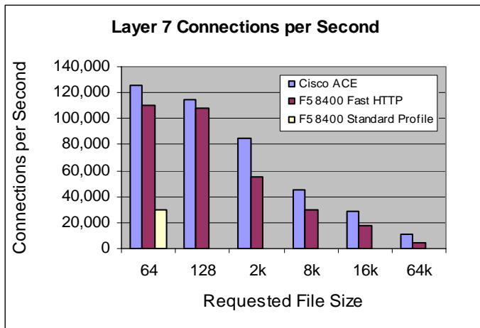
Chart 3: L7 CPS over Various File Sizes
