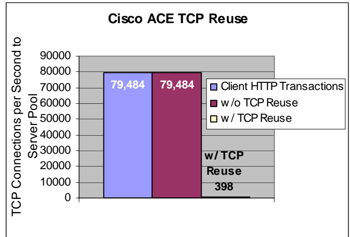
Chart 8: Cisco ACE TCP Reuse test results
