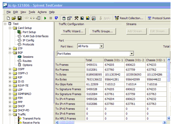
Figure 1: Screenshot of four ACE modules with 1500 byte traffic at 60+ Rx Gbps rate.
